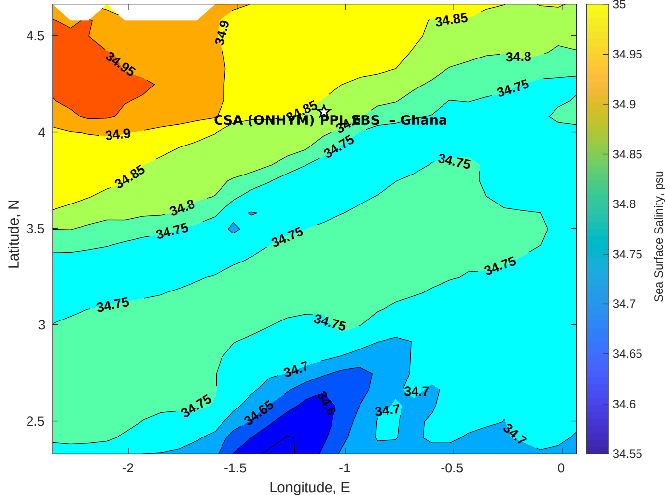
Surface Salinity for CSA (ONHYM) PPL EBS - Ghana at 22-May-2025 00:00:00
