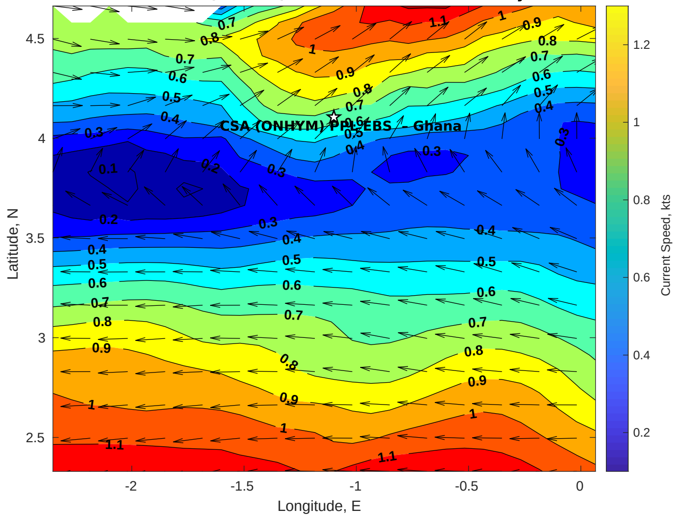
Surface Currents for CSA (ONHYM) PPL EBS - Ghana at 22-May-2025 00:00:00
