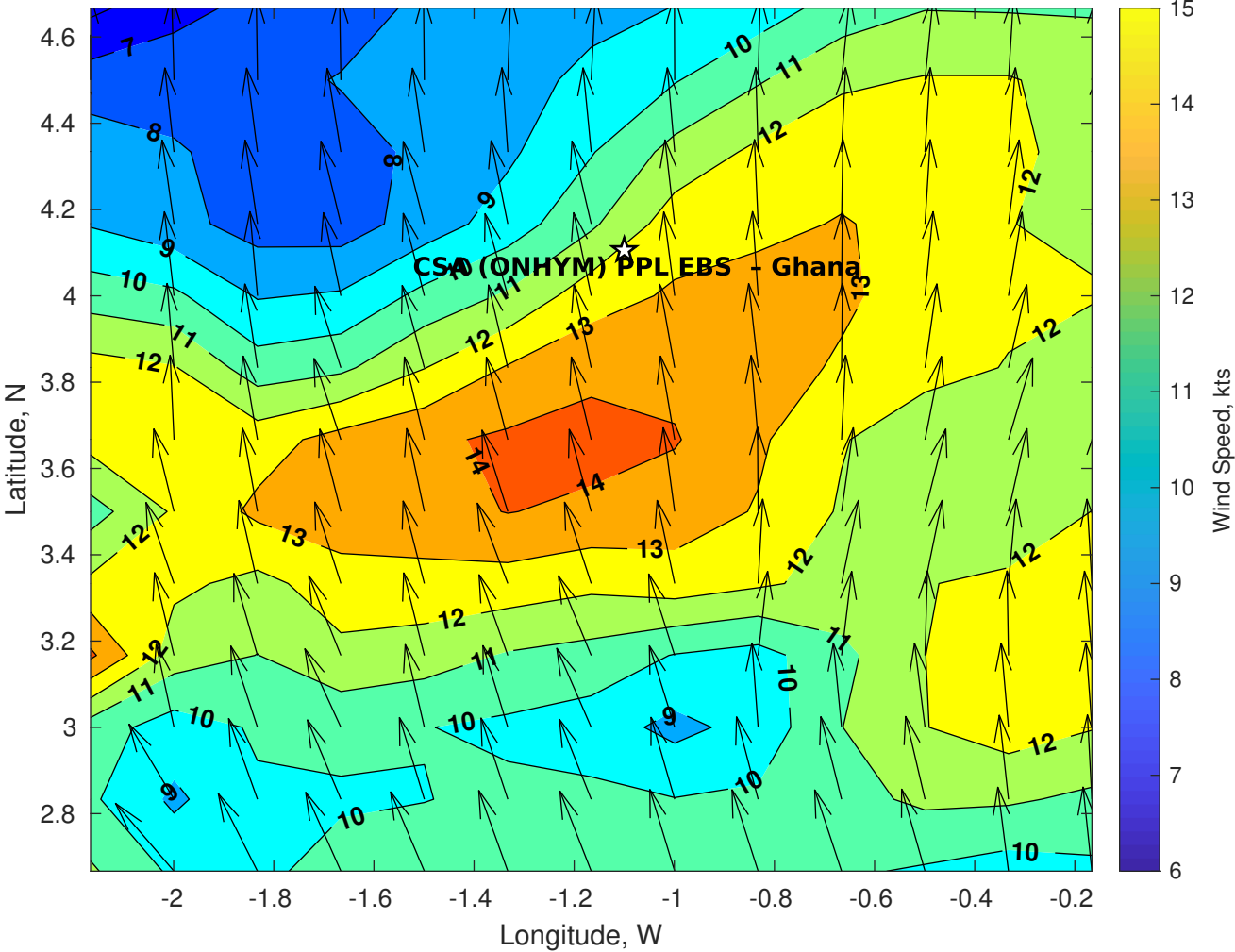
Winds (kts) for CSA (ONHYM) PPL EBS - Ghana at 23-May-2025 09:00:00
