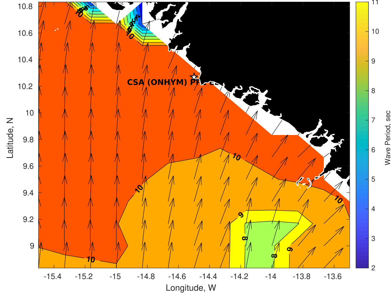
Wave Period (sec) for CSA (ONHYM) PPL EBS - Guinea at 23-May-2025 09:00:00
