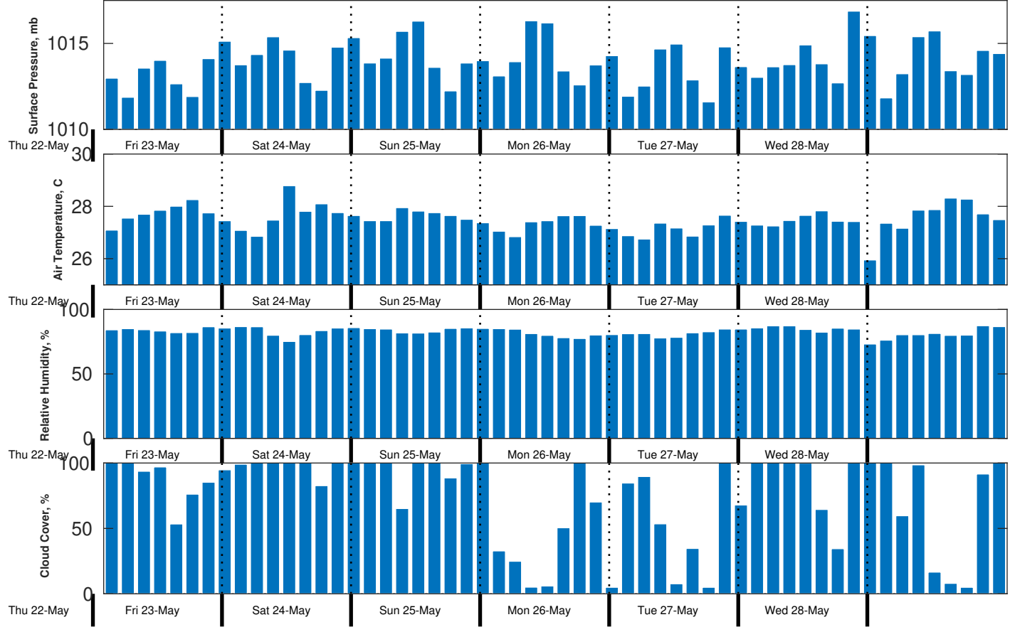
Met Forecast for CSA (ONHYM) PPL EBS - Guinea from 23-May-2025 00:00:00 to 30-May-2025 00:00:00
