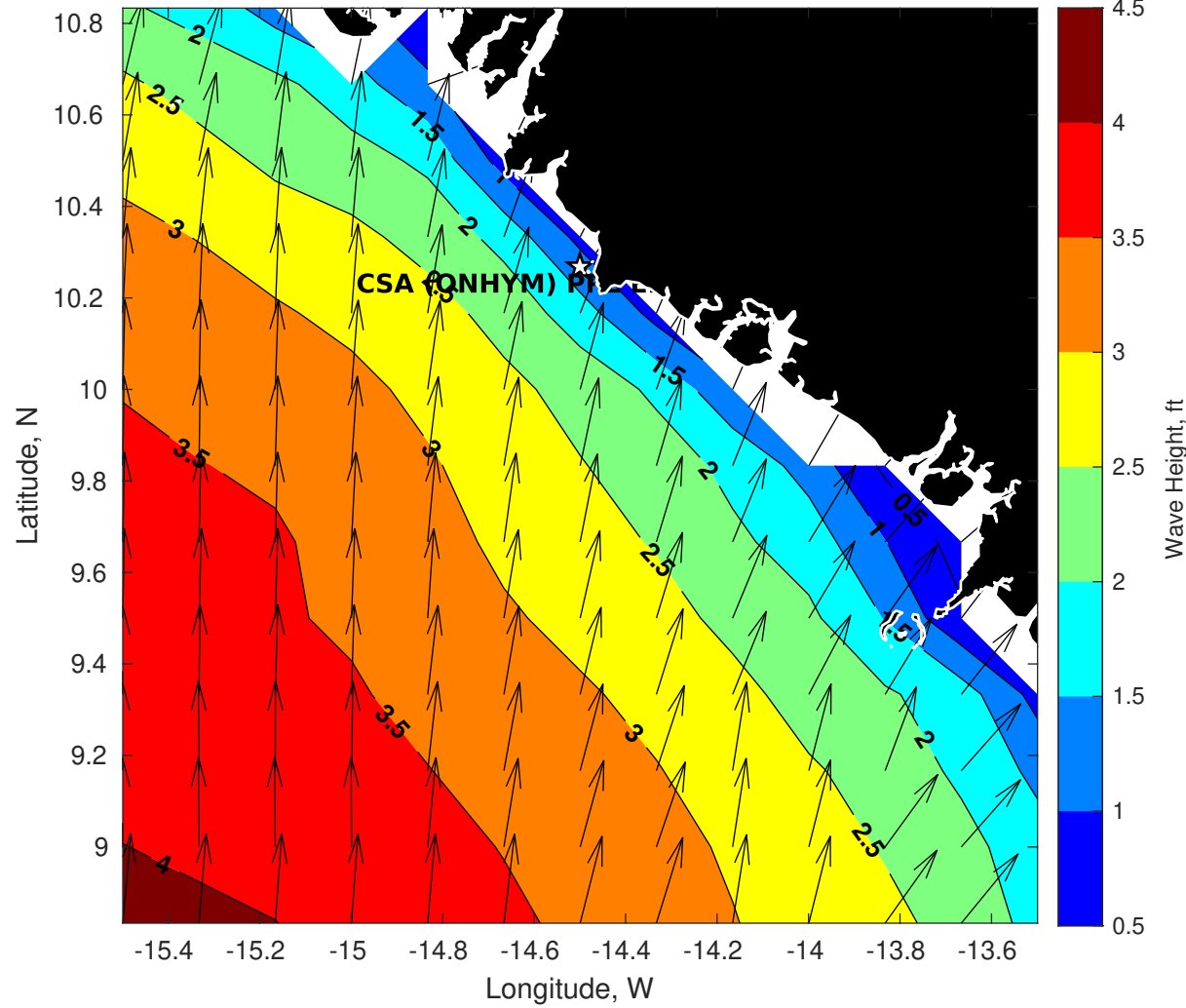
Wave Height (ft) for CSA (ONHYM) PPL EBS - Guinea at 23-May-2025 09:00:00
