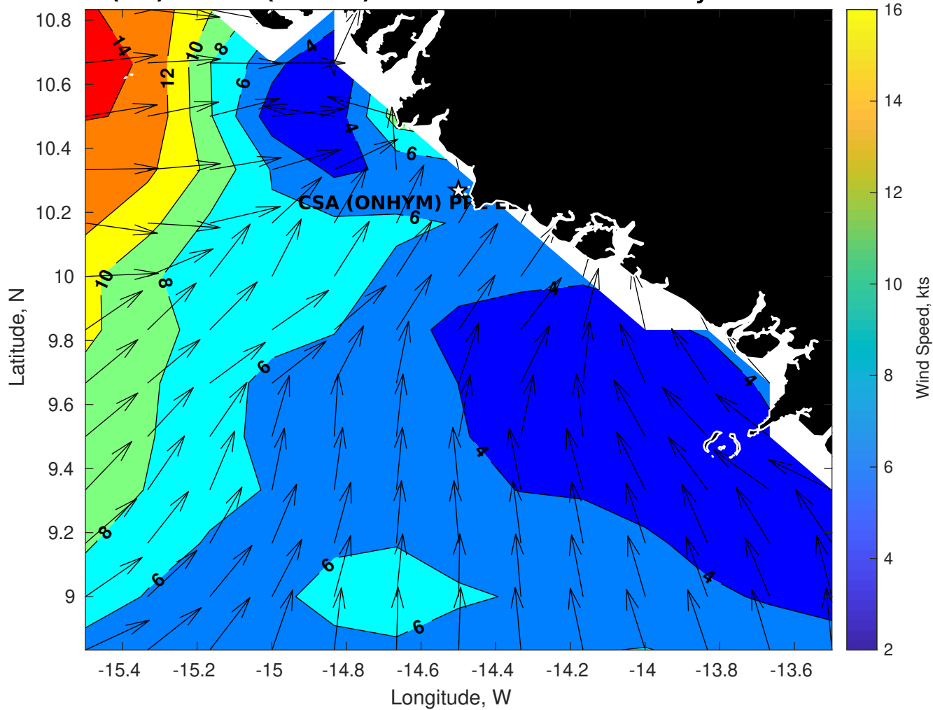
Winds (kts) for CSA (ONHYM) PPL EBS - Guinea at 23-May-2025 09:00:00
