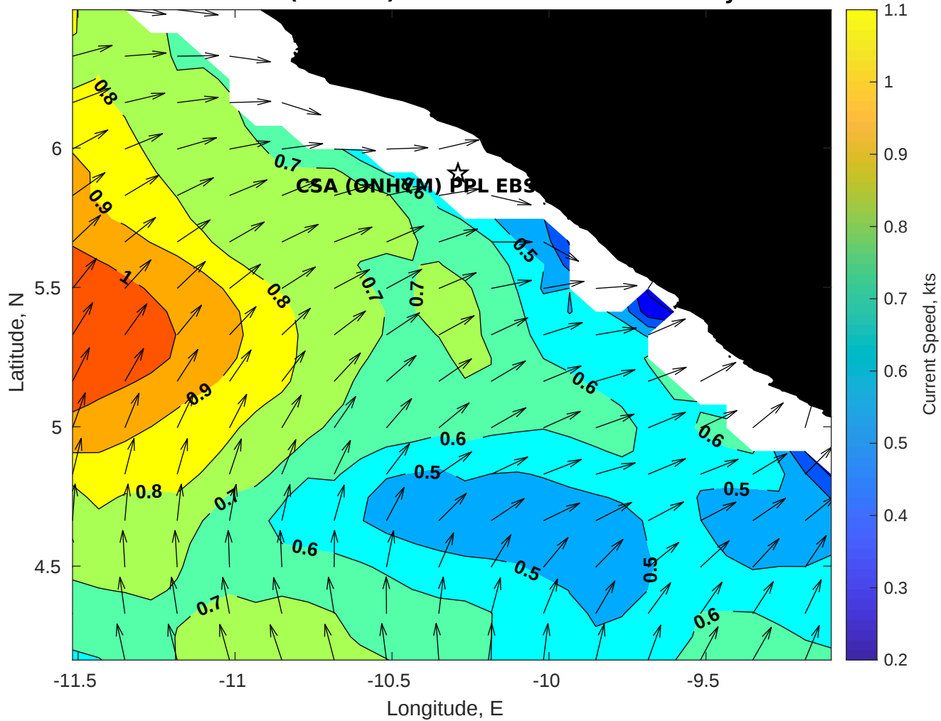
Surface Currents for CSA (ONHYM) PPL EBS - Liberia at 22-May-2025 00:00:00
