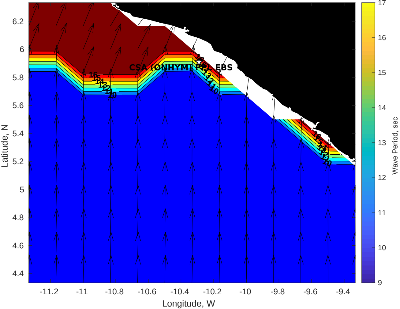
Wave Period (sec) for CSA (ONHYM) PPL EBS - Liberia at 23-May-2025 09:00:00
