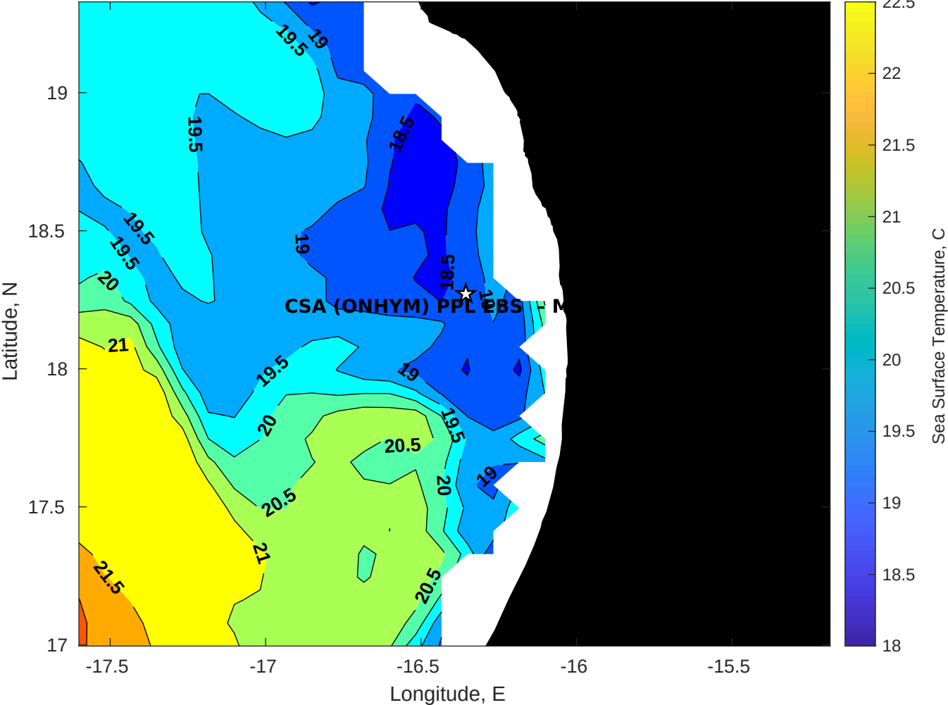
SST for CSA (ONHYM) PPL EBS - Mauritania at 22-May-2025 00:00:00
