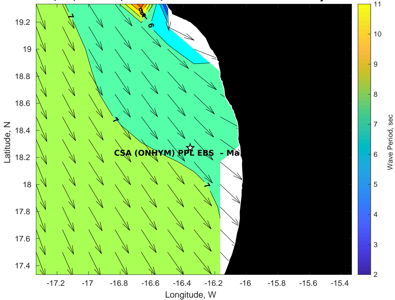
Wave Period (sec) for CSA (ONHYM) PPL EBS - Mauritania at 23-May-2025 09:00:00
