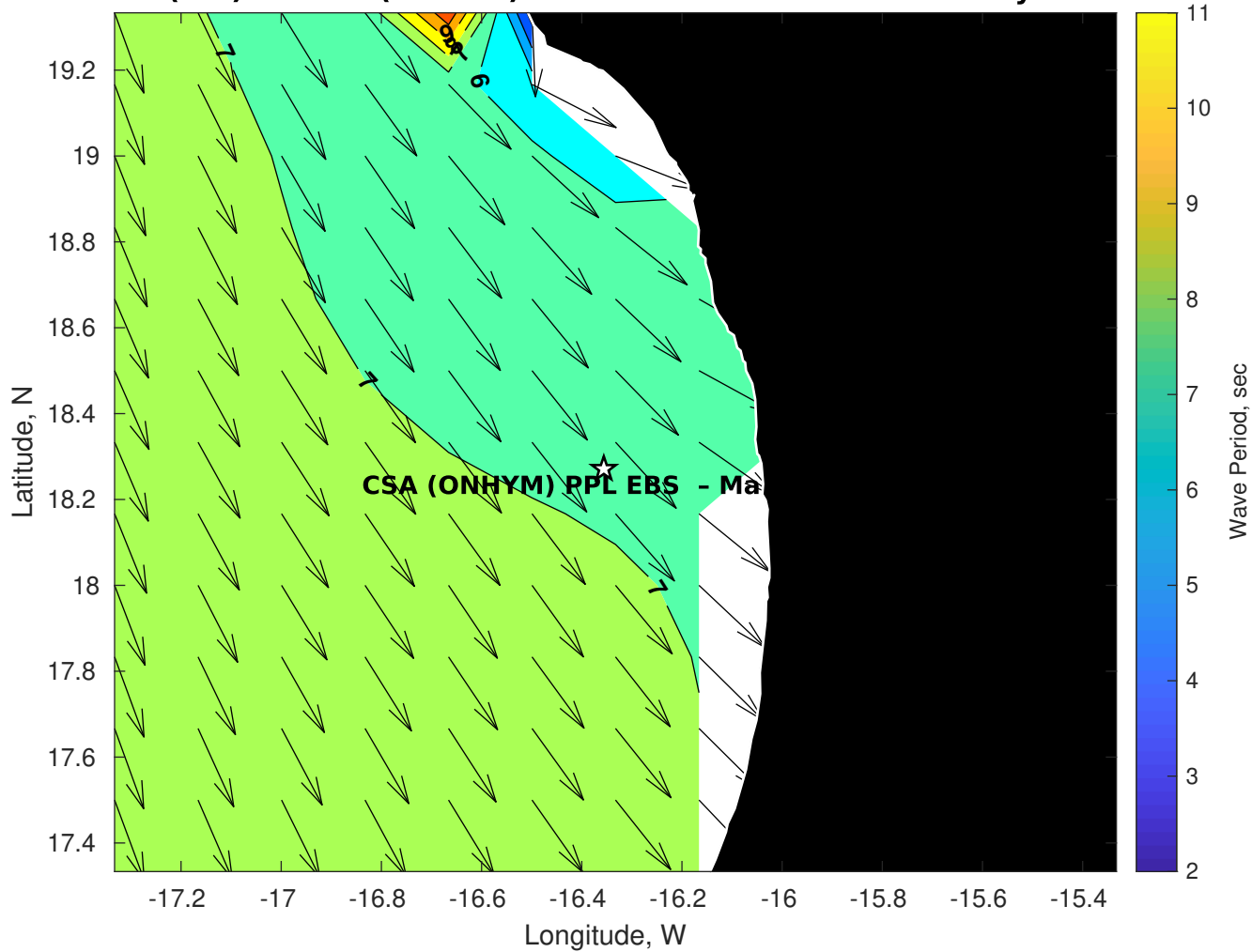
Wave Period (sec) for CSA (ONHYM) PPL EBS - Mauritania at 23-May-2025 09:00:00
