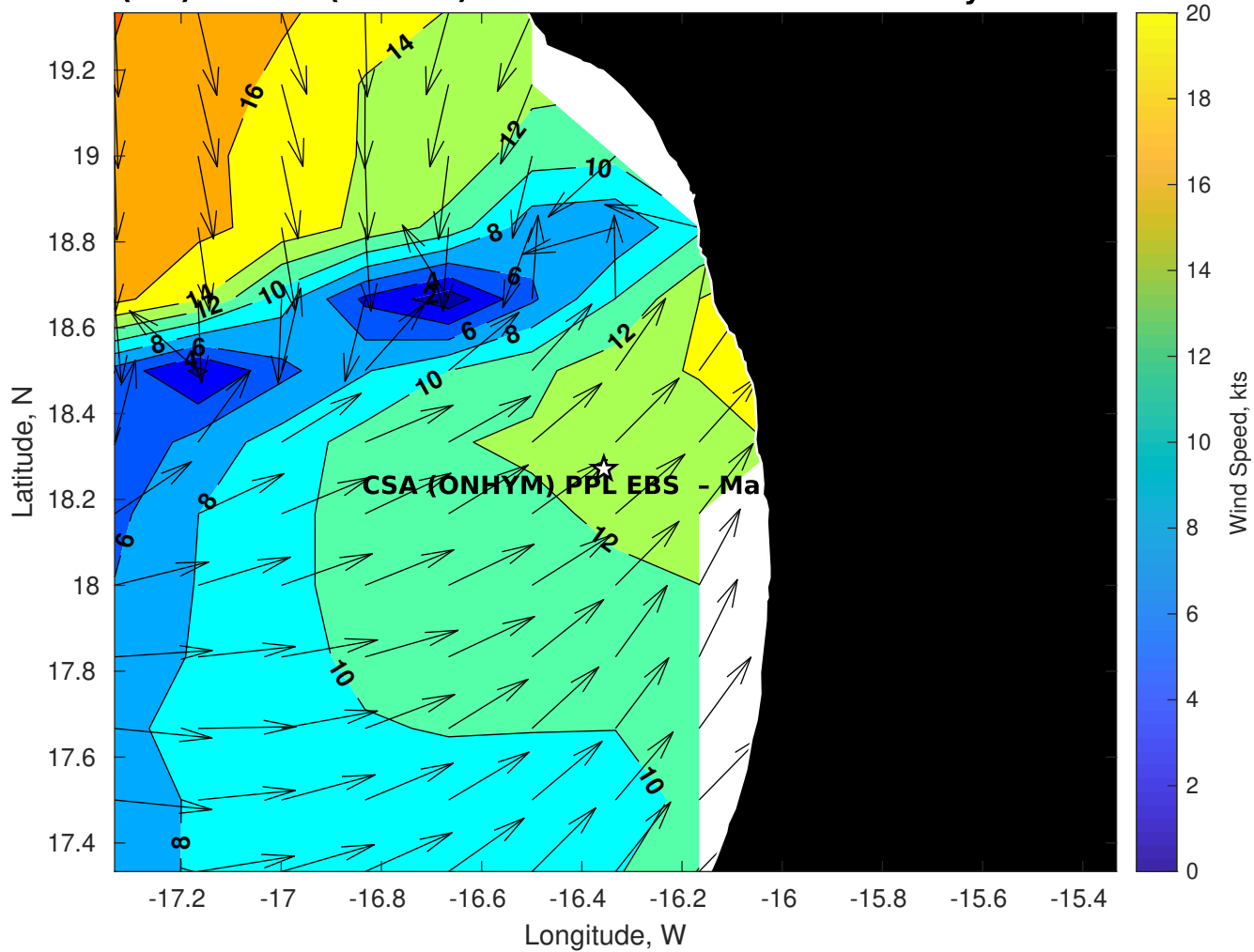
Winds (kts) for CSA (ONHYM) PPL EBS - Mauritania at 23-May-2025 09:00:00
