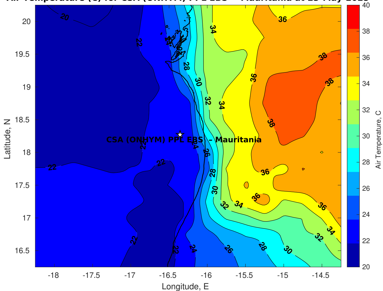
Air Temperature (C) for CSA (ONHYM) PPL EBS - Mauritania at 23-May-2025
