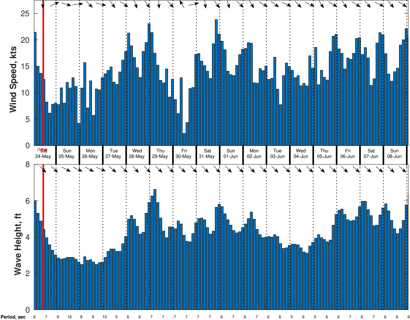
Wind & Wave Forecast for CSA (ONHYM) PPL EBS - Mauritania from 23-May-2025 01:00:00 to 08-Jun-2025 01:00:00
