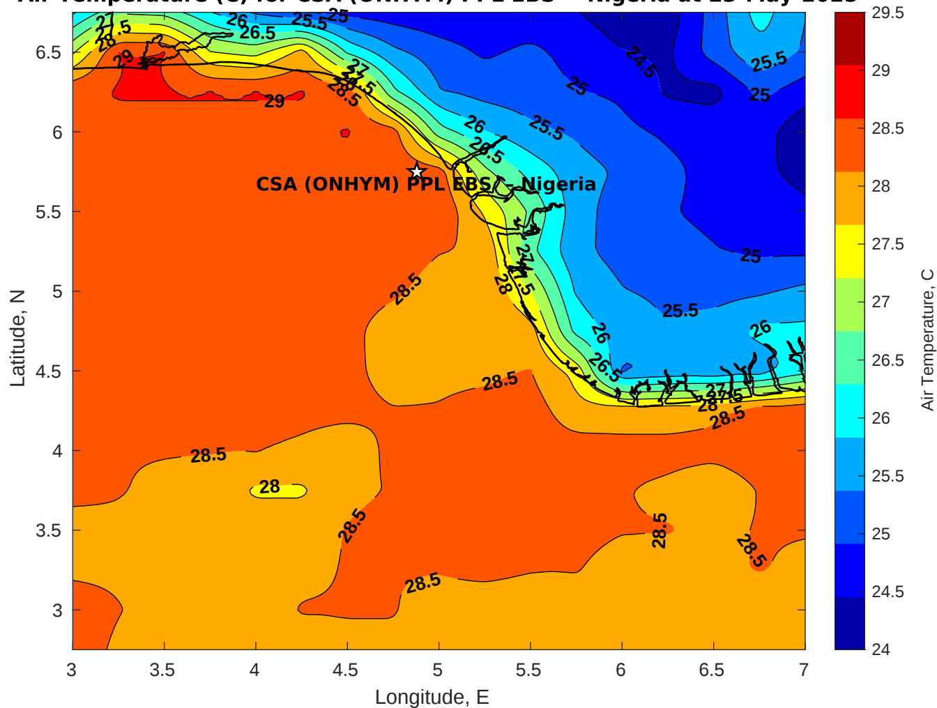
Air Temperature (C) for CSA (ONHYM) PPL EBS - Nigeria at 23-May-2025
