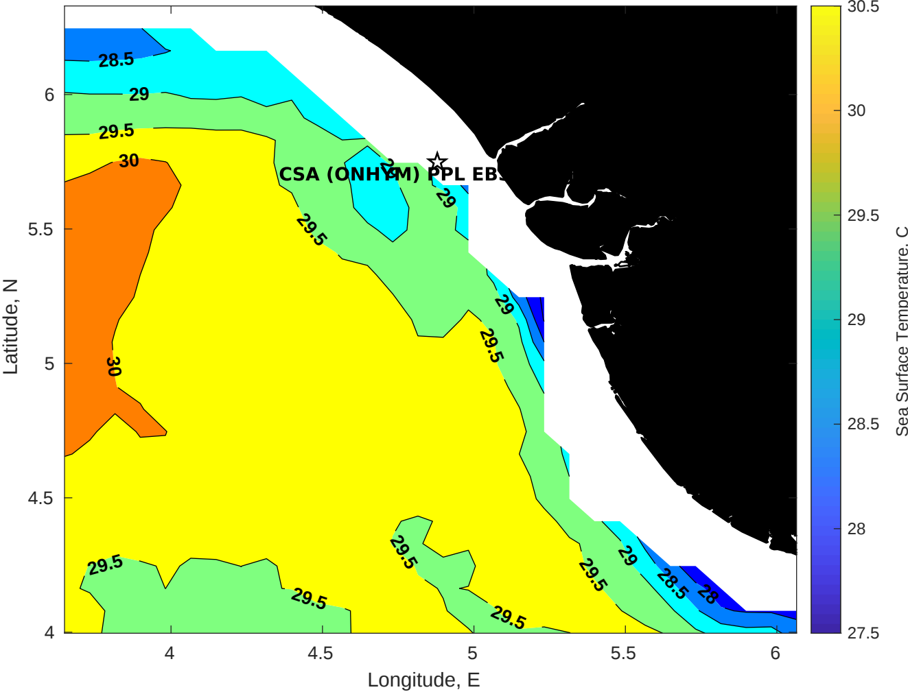
SST for CSA (ONHYM) PPL EBS - Nigeria at 22-May-2025 00:00:00
