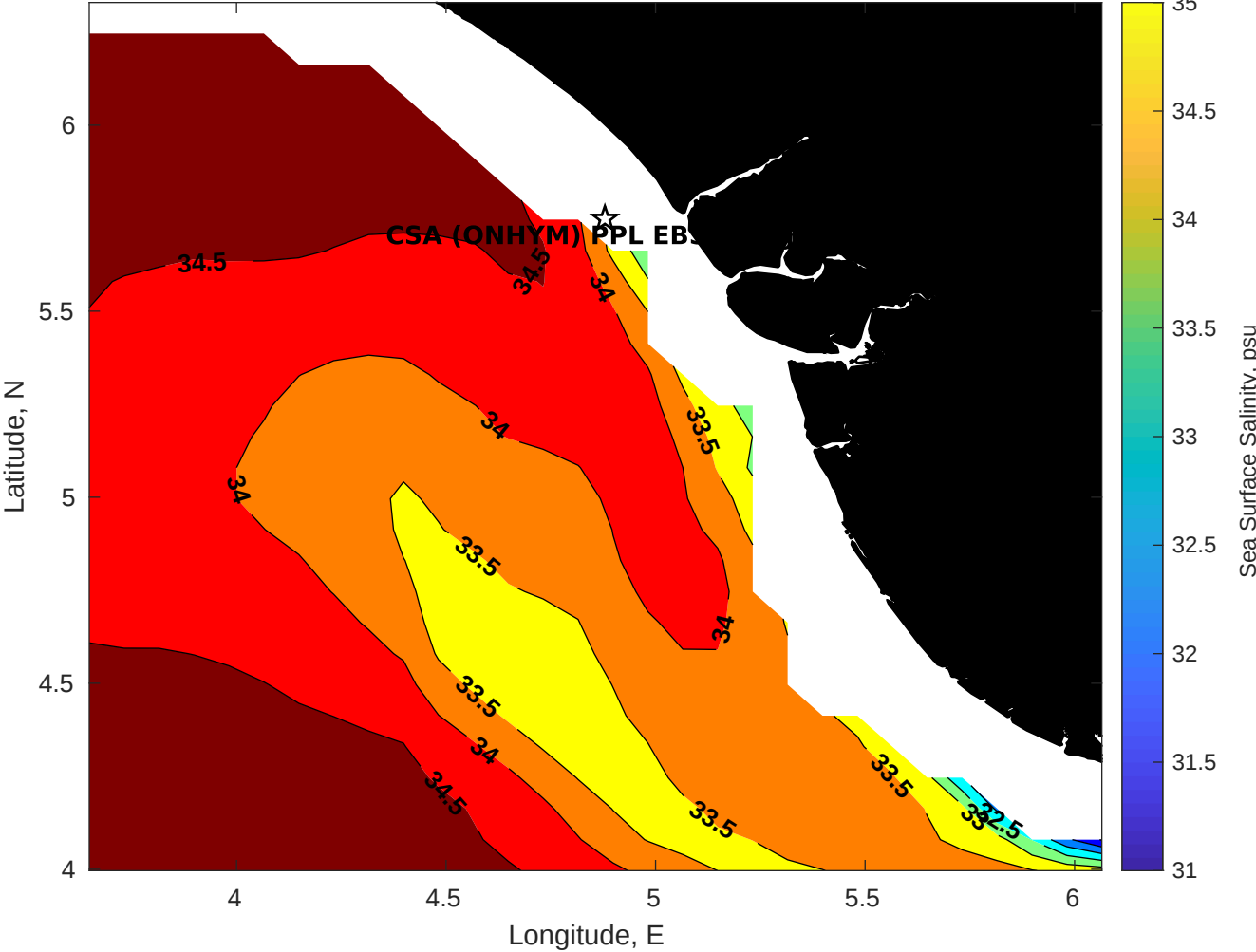
Surface Salinity for CSA (ONHYM) PPL EBS - Nigeria at 22-May-2025 00:00:00
