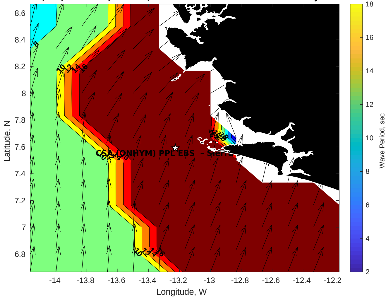
Wave Period (sec) for CSA (ONHYM) PPL EBS - Sierra Leone at 23-May-2025 09:00:00
