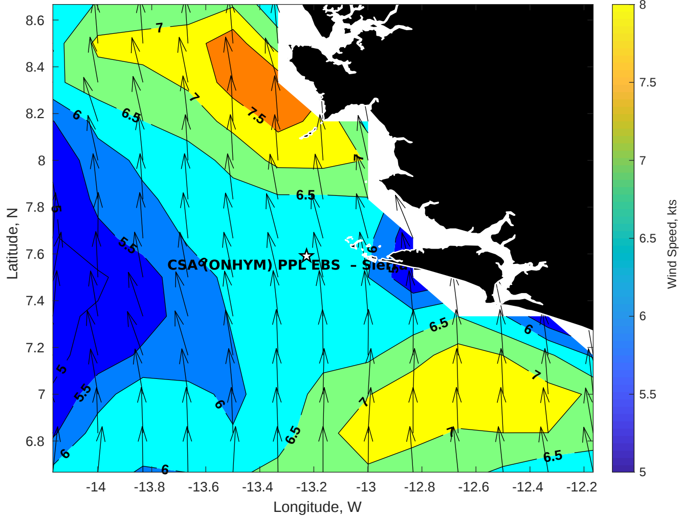
Winds (kts) for CSA (ONHYM) PPL EBS - Sierra Leone at 23-May-2025 09:00:00
