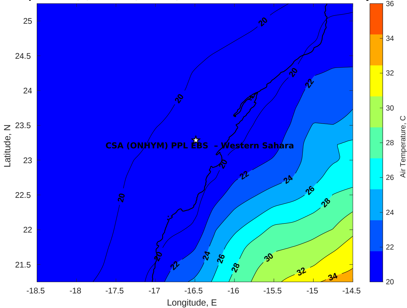
Air Temperature (C) for CSA (ONHYM) PPL EBS - Western Sahara at 23-May-2025
