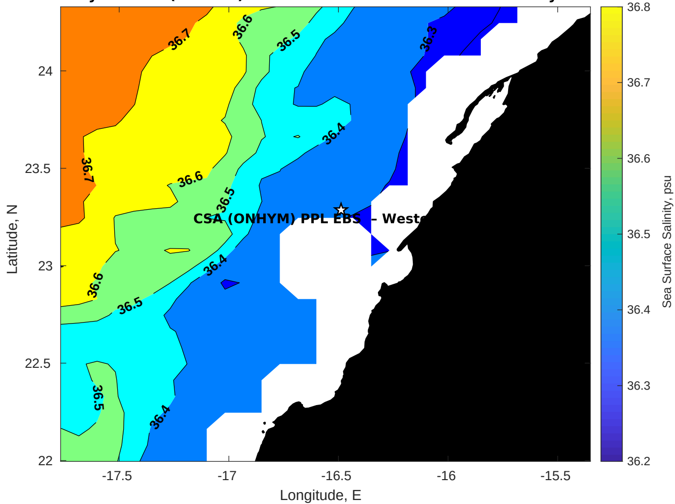
Surface Salinity for CSA (ONHYM) PPL EBS - Western Sahara at 22-May-2025 00:00:00
