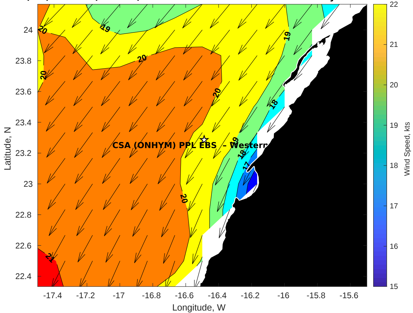
Winds (kts) for CSA (ONHYM) PPL EBS - Western Sahara at 23-May-2025 09:00:00
