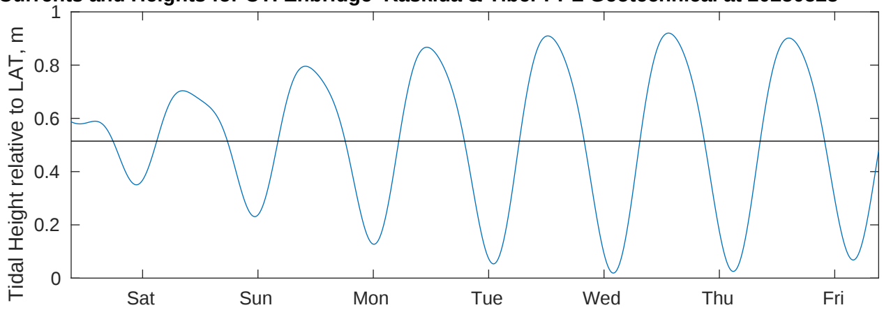
Tidal Currents and Heights for CTI Enbridge Kaskida & Tiber PPL Geotechnical at 20250523
