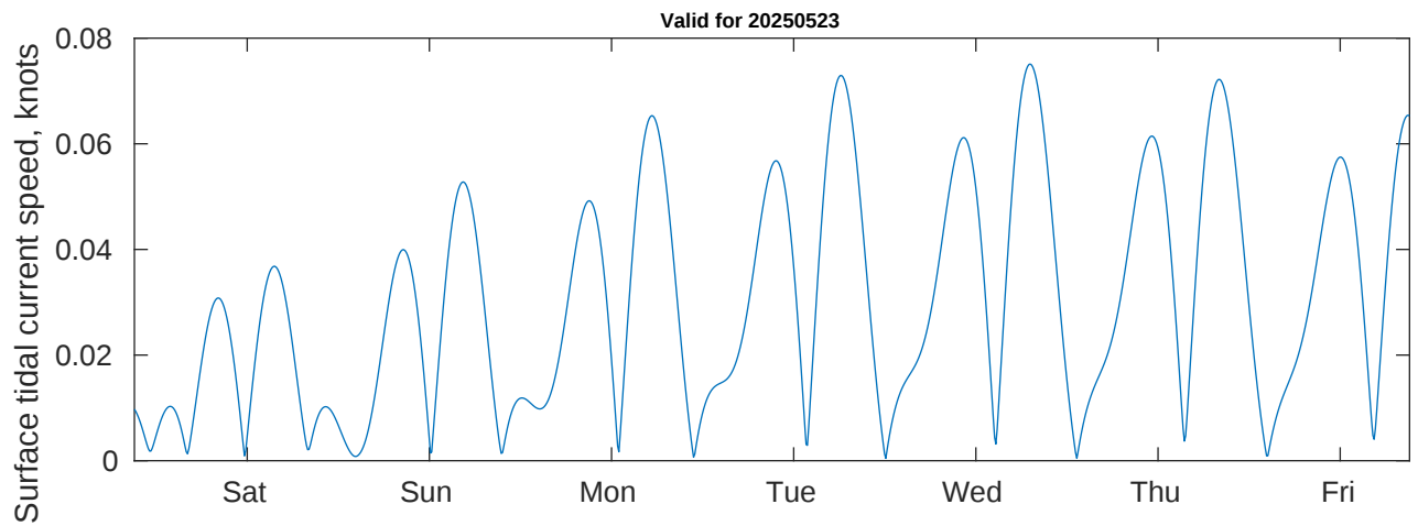
Tidal Currents and Heights for CTI Enbridge Kaskida & Tiber PPL Geotechnical at 20250523
