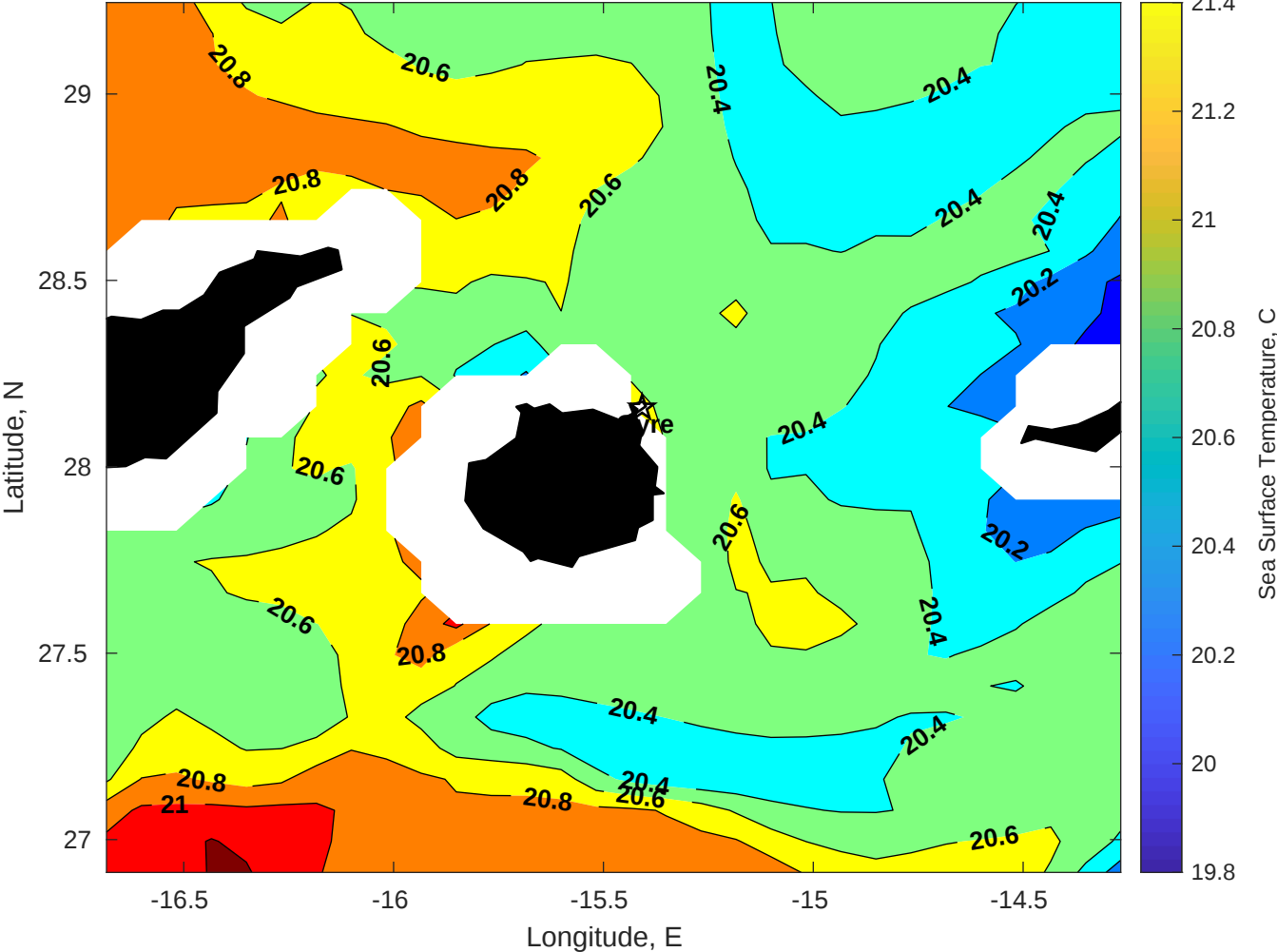
SST for Gyre at 22-May-2025 00:00:00
