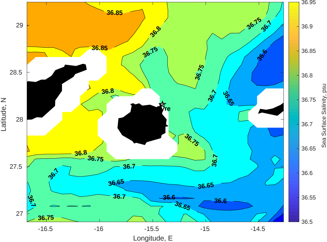
Surface Salinity for Gyre at 22-May-2025 00:00:00
