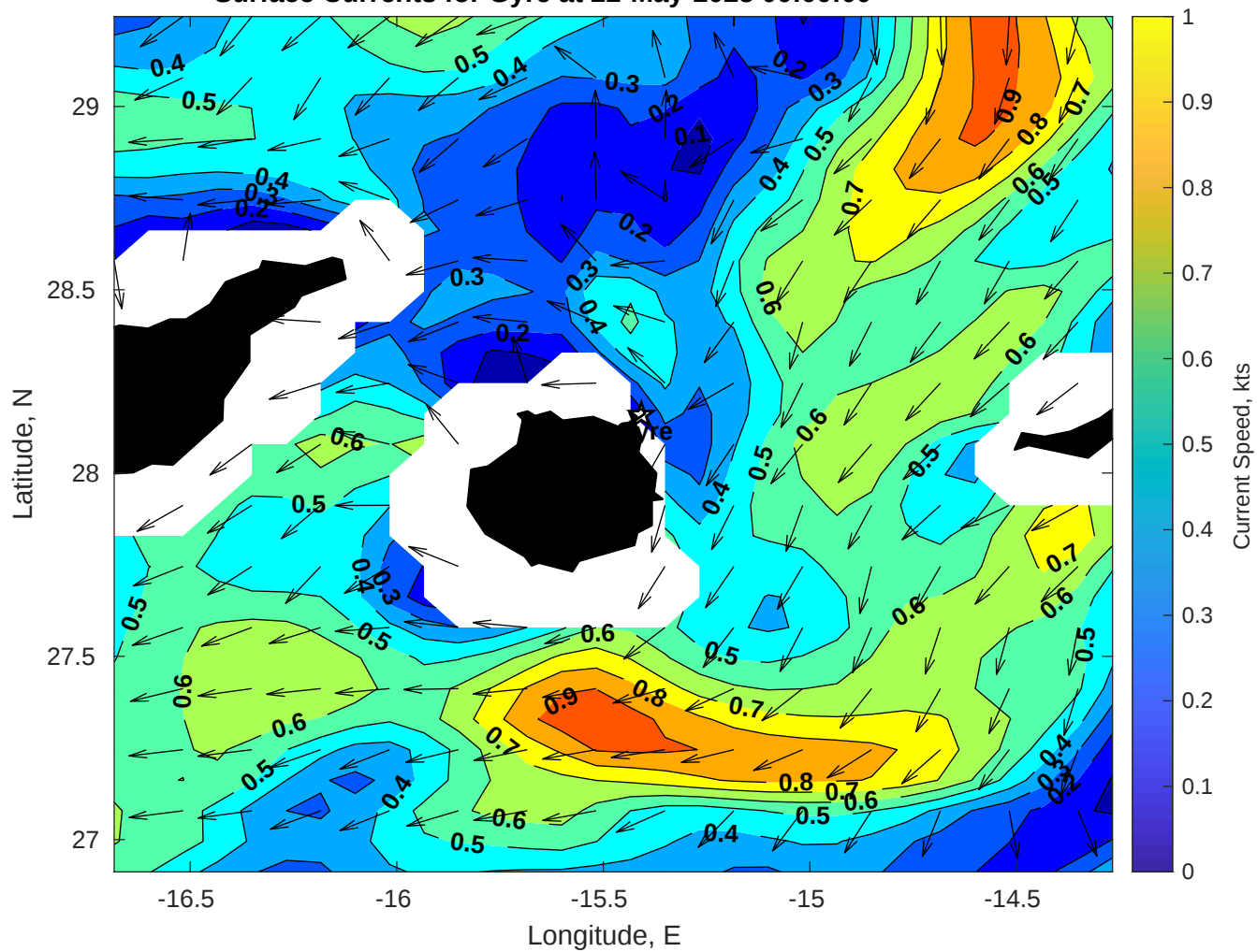
Surface Currents for Gyre at 22-May-2025 00:00:00
