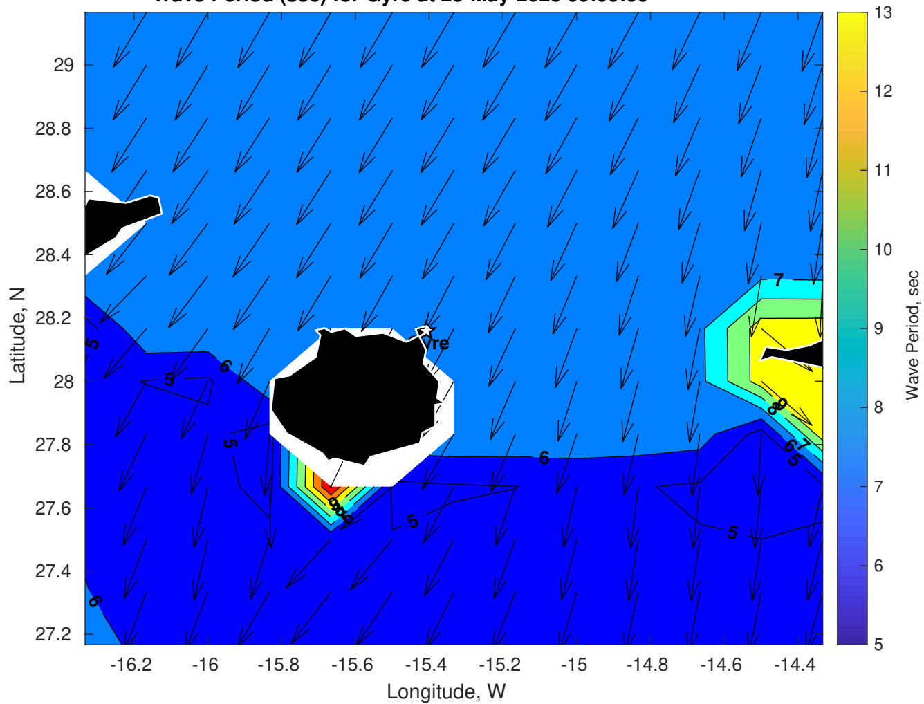
Wave Period (sec) for Gyre at 23-May-2025 09:00:00
