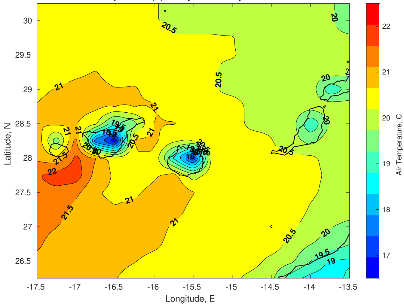
Air Temperature (C) for Gyre at 23-May-2025
