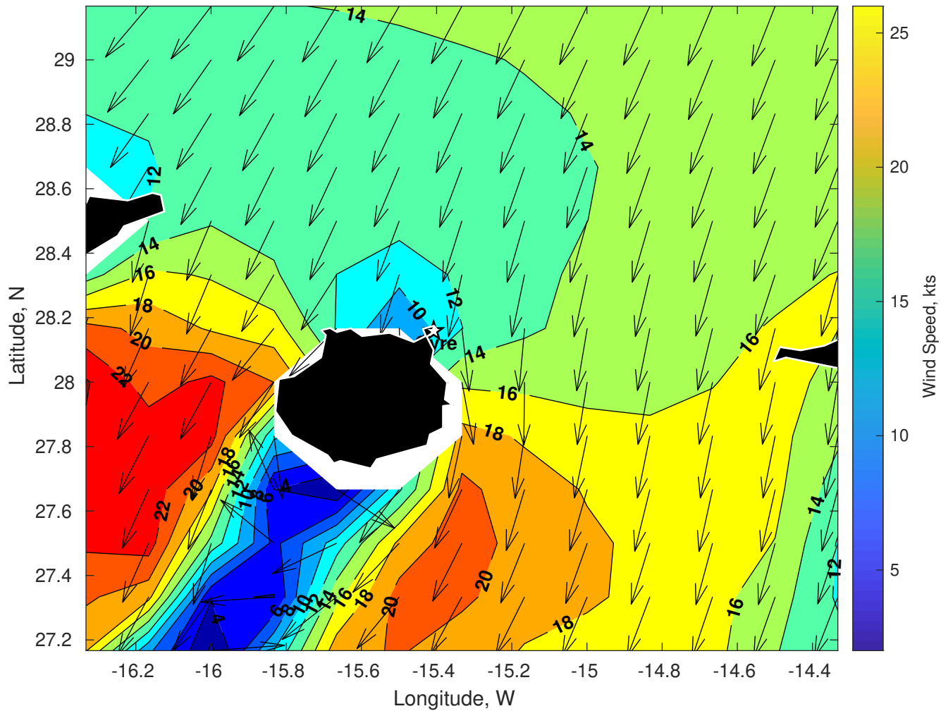
Winds (kts) for Gyre at 23-May-2025 09:00:00
