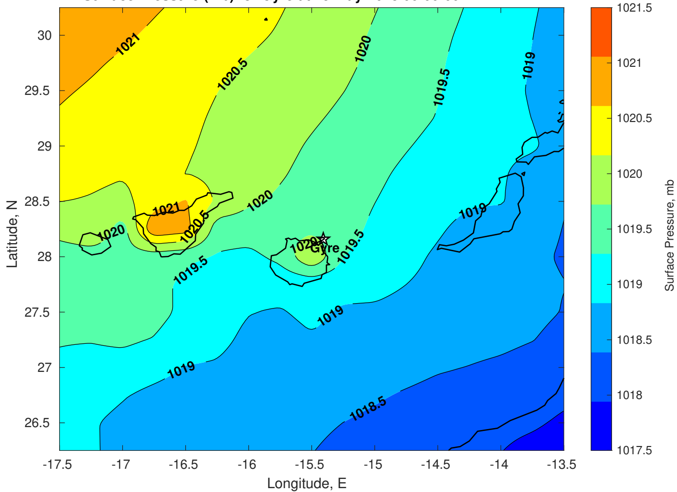
Surface Pressure (mb) for Gyre at 25-May-2025 00:00:00
