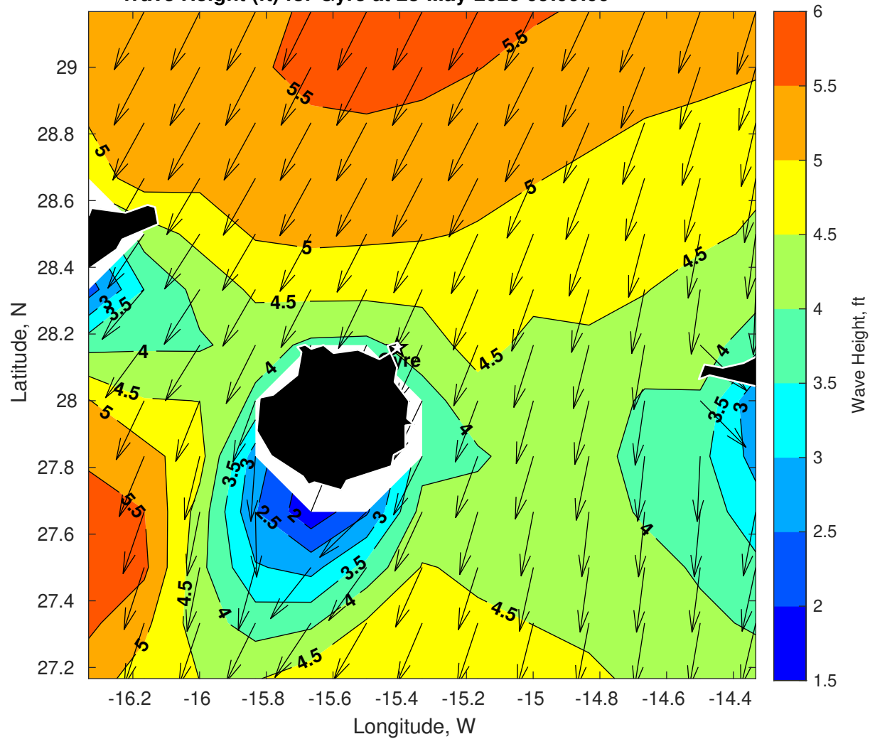
Wave Height (ft) for Gyre at 23-May-2025 09:00:00
