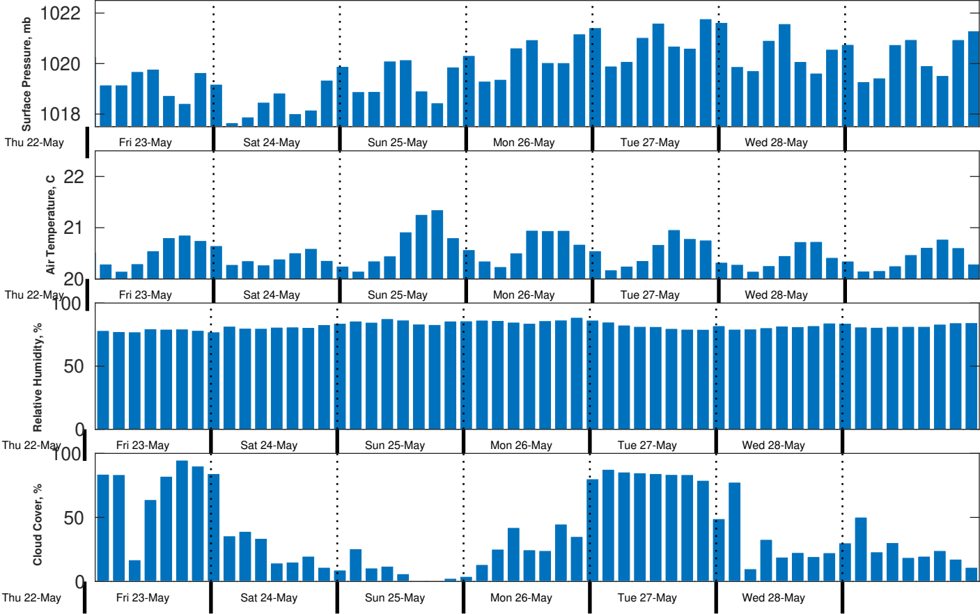
Met Forecast for Gyre from 22-May-2025 23:00:00 to 29-May-2025 23:00:00
