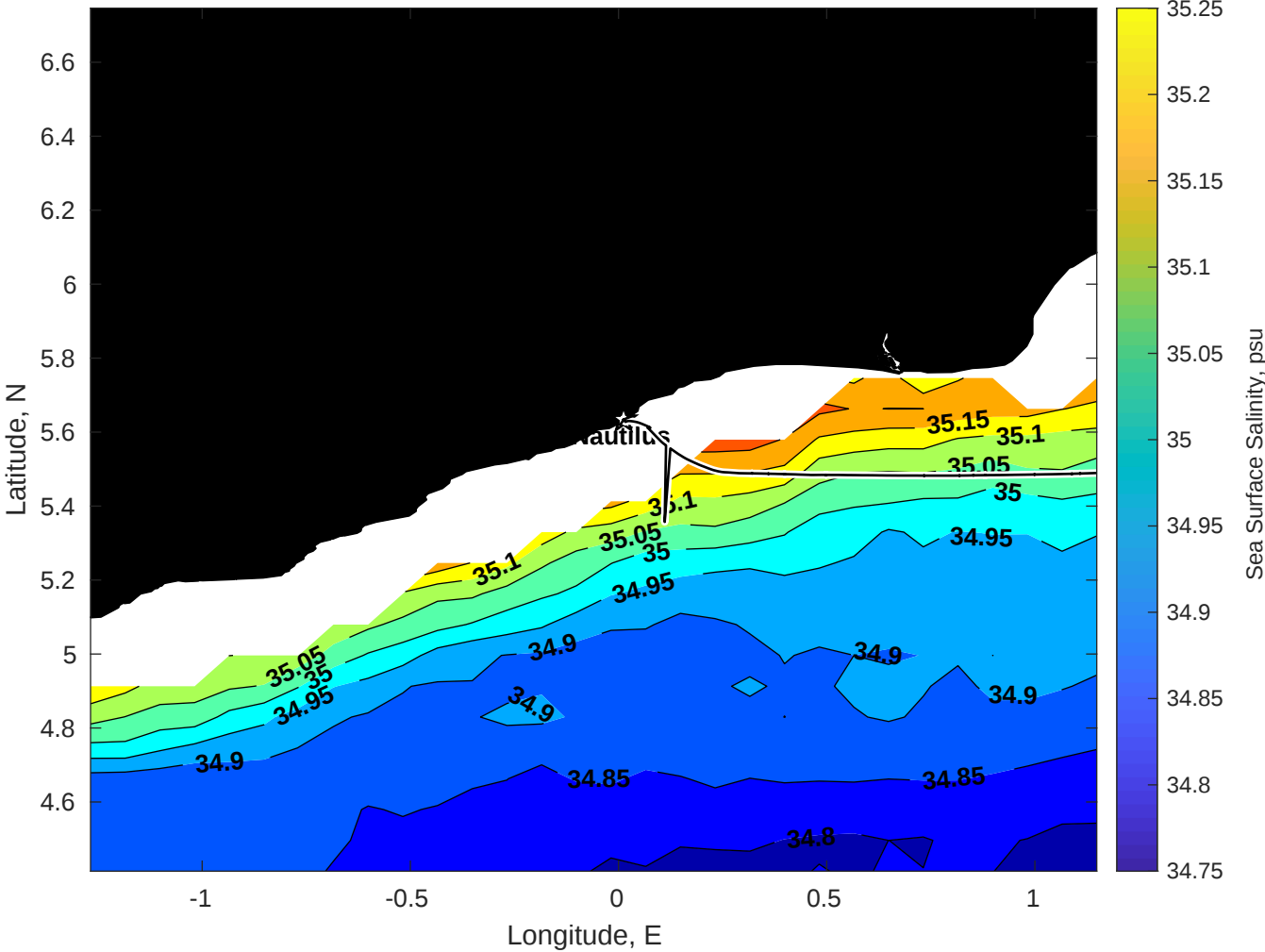
Surface Salinity for Nautilus at 22-May-2025 00:00:00
