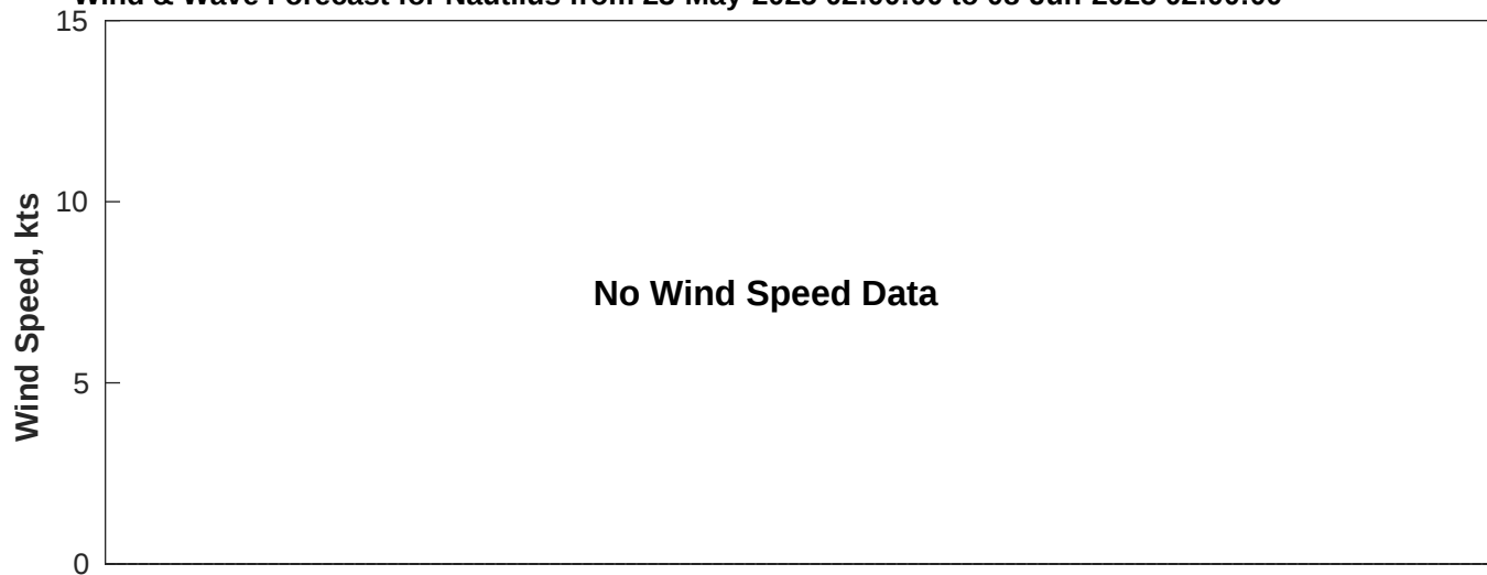
Wind & Wave Forecast for Nautilus from 23-May-2025 02:00:00 to 08-Jun-2025 02:00:00
