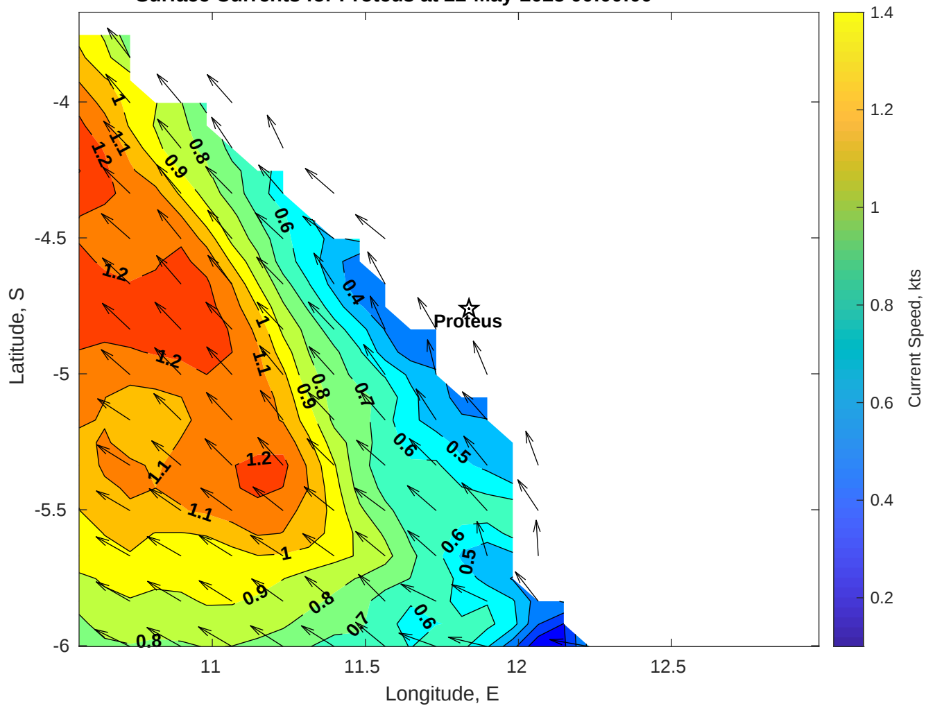
Surface Currents for Proteus at 22-May-2025 00:00:00
