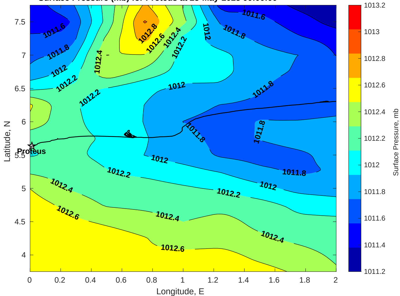
Surface Pressure (mb) for Proteus at 23-May-2025 00:00:00
