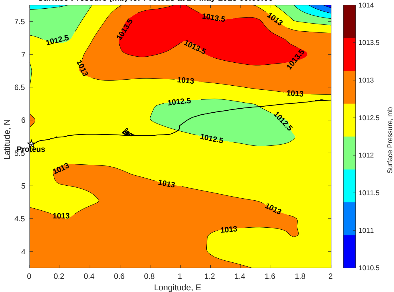
Surface Pressure (mb) for Proteus at 24-May-2025 00:00:00
