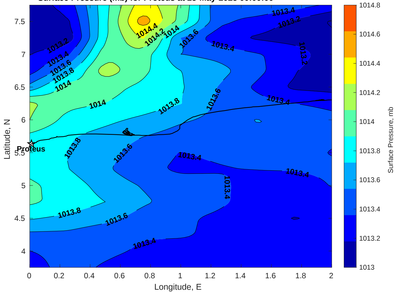
Surface Pressure (mb) for Proteus at 25-May-2025 00:00:00
