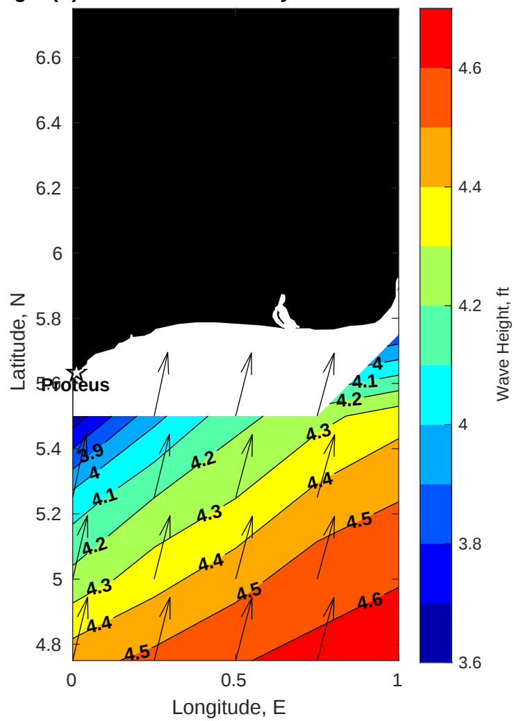
Wave Height (ft) for Proteus at 23-May-2025 09:00:00
