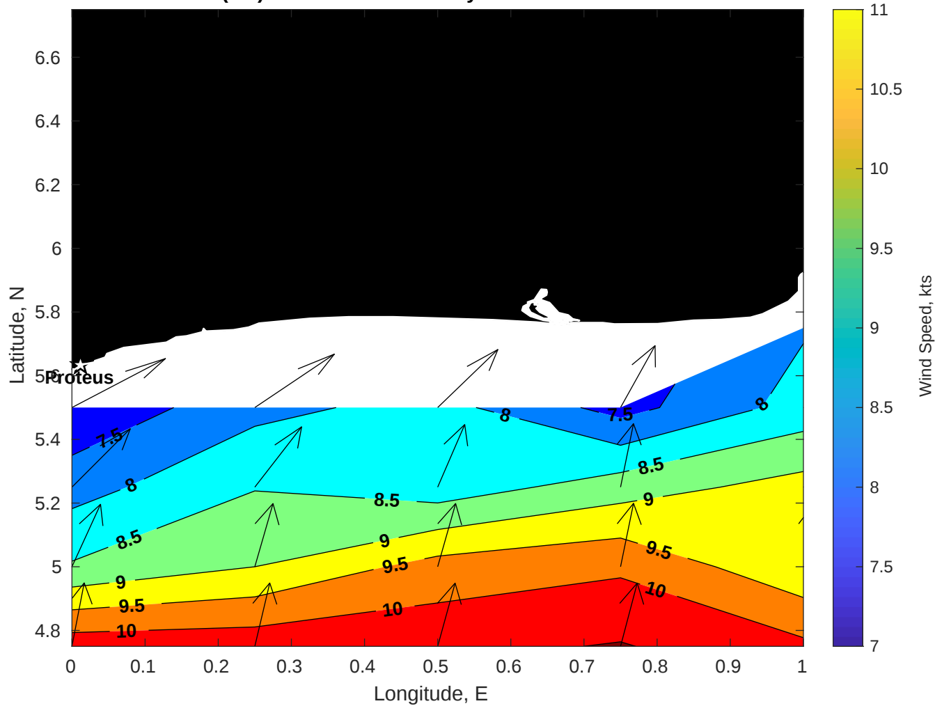
Winds (kts) for Proteus at 23-May-2025 09:00:00
