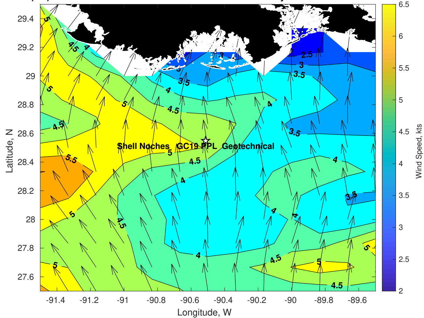
Winds (kts) for Shell Noches GC19 PPL Geotechnical at 23-May-2025 09:00:00
