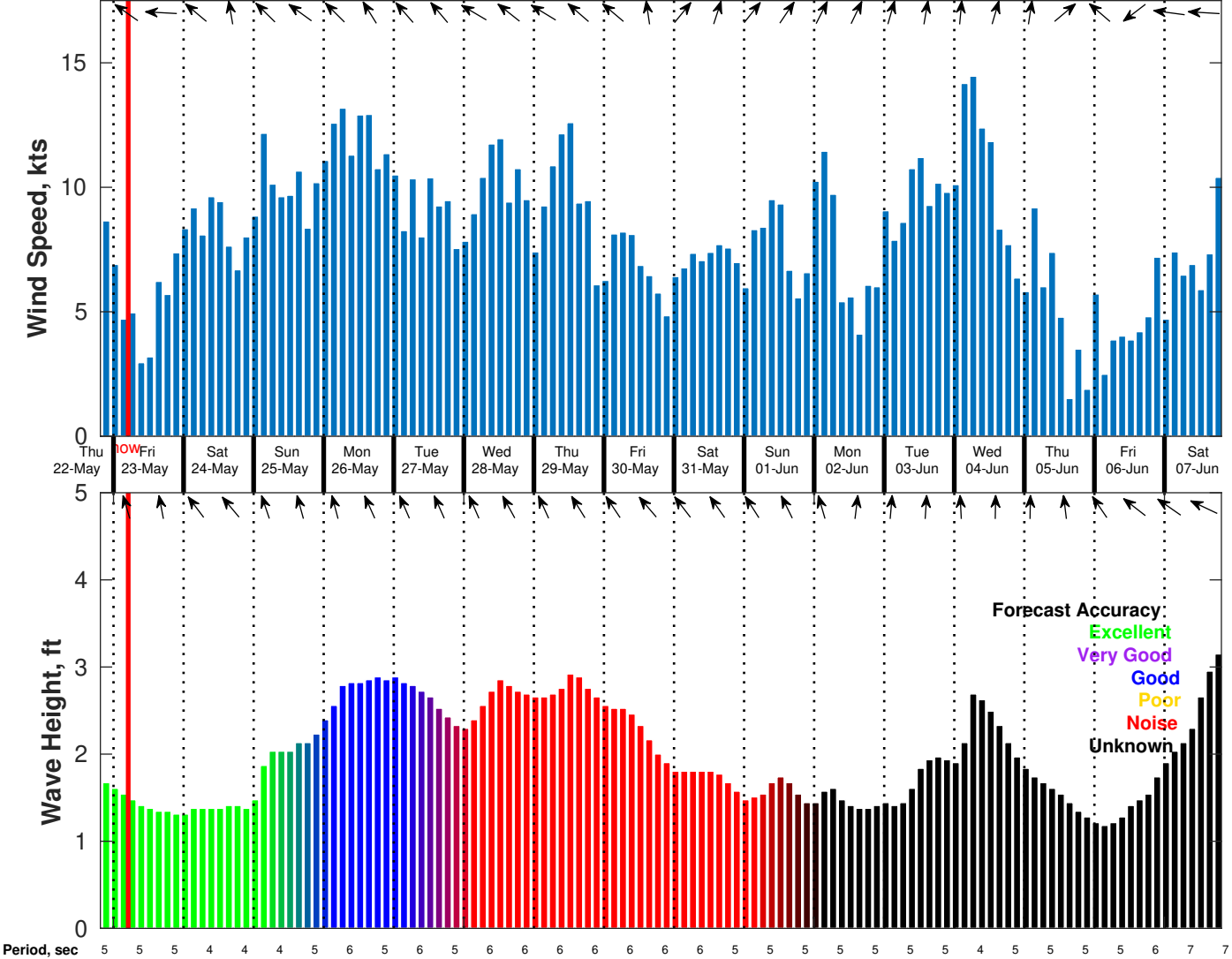
Wind & Wave Forecast for Shell Noches GC19 PPL Geotechnical from 22-May-2025 20:00:00 to 07-Jun-2025 20:00:00
