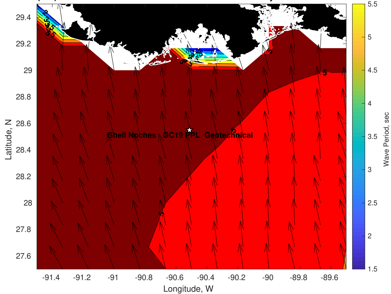
Wave Period (sec) for Shell Noches GC19 PPL Geotechnical at 23-May-2025 09:00:00
