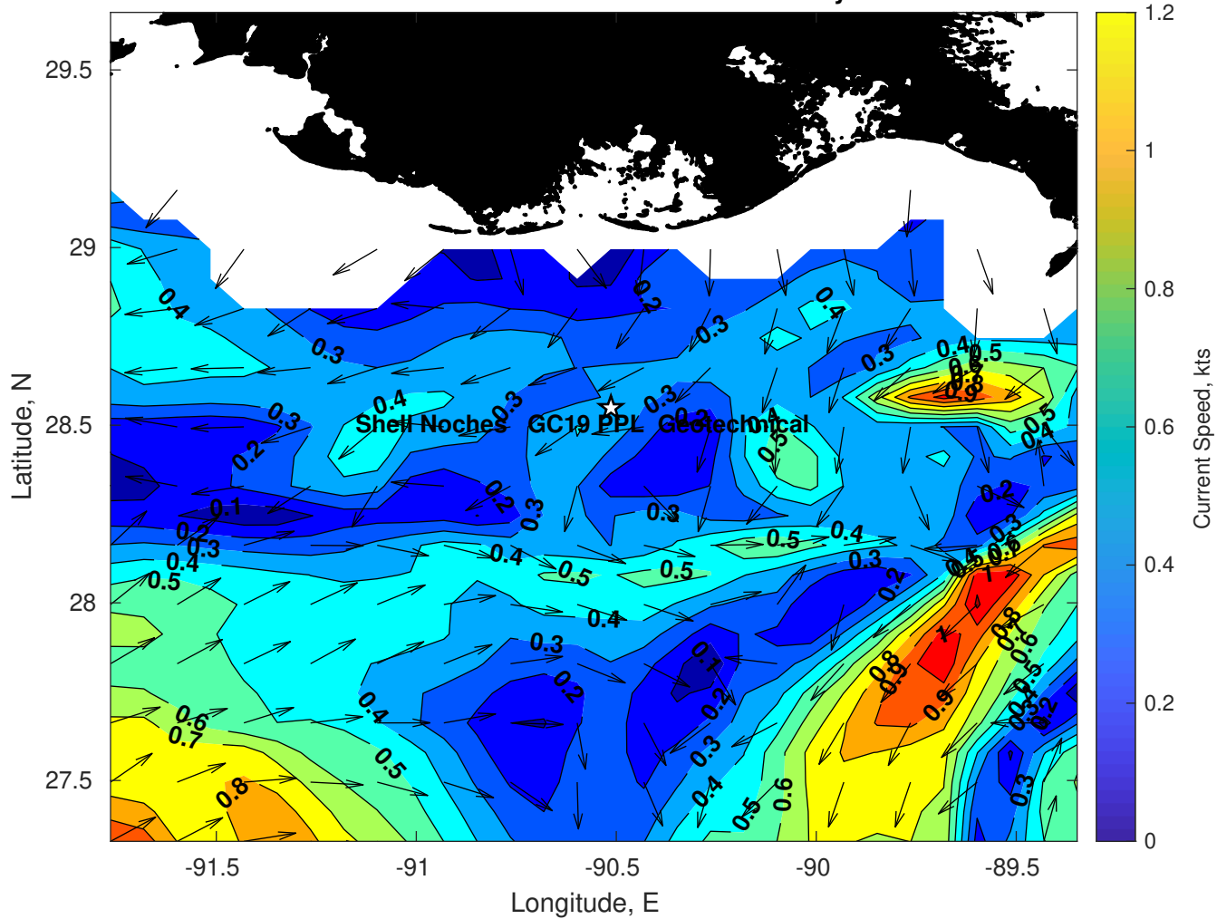
Surface Currents for Shell Noches GC19 PPL Geotechnical at 22-May-2025 00:00:00
