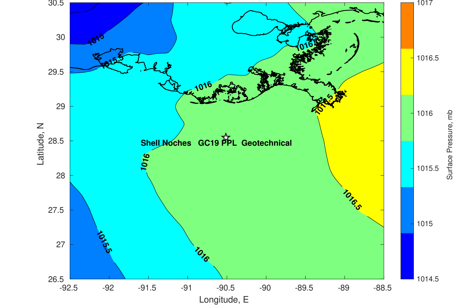
Surface Pressure (mb) for Shell Noches GC19 PPL Geotechnical at 24-May-2025 00:00:00
