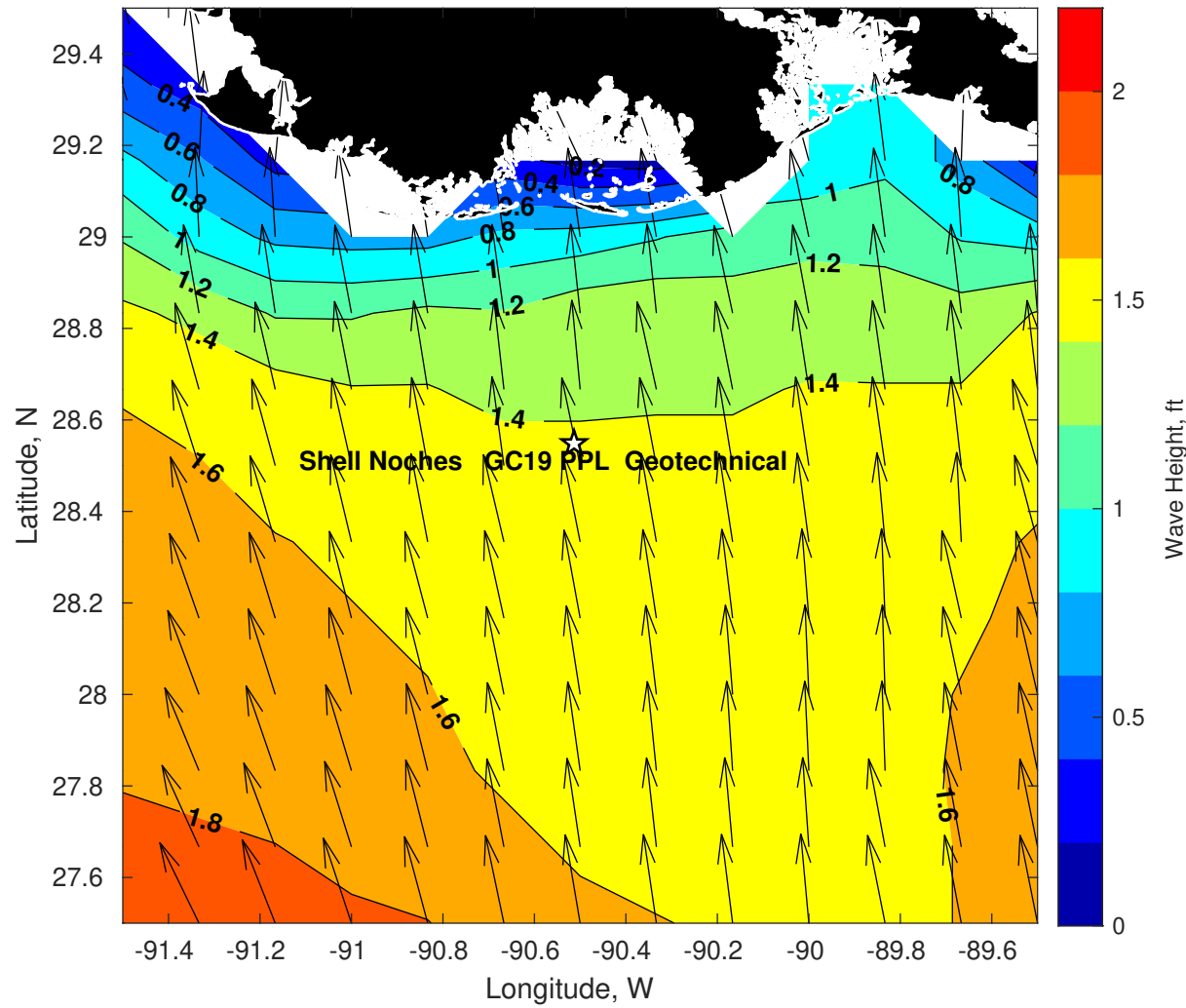
Wave Height (ft) for Shell Noches GC19 PPL Geotechnical at 23-May-2025 09:00:00
