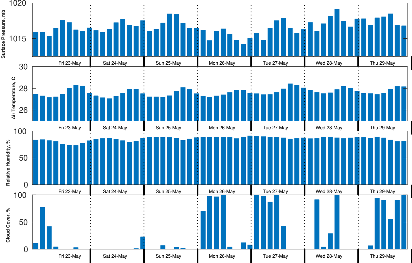
Met Forecast for Shell Noches GC19 PPL Geotechnical from 23-May-2025 00:00:00 to 30-May-2025 00:00:00
