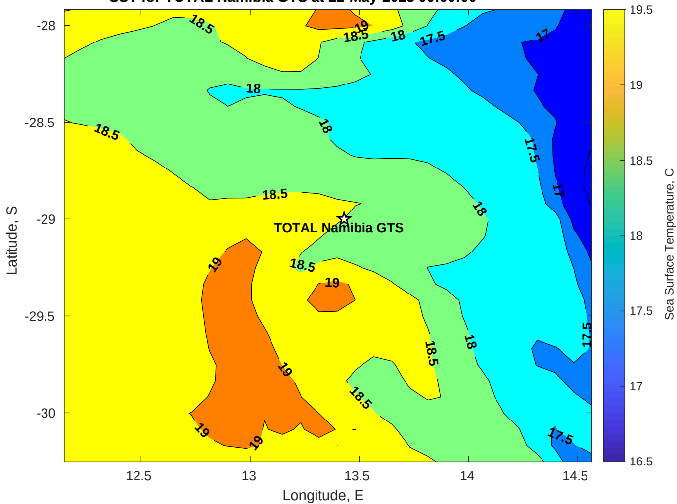
SST for TOTAL Namibia GTS at 22-May-2025 00:00:00
