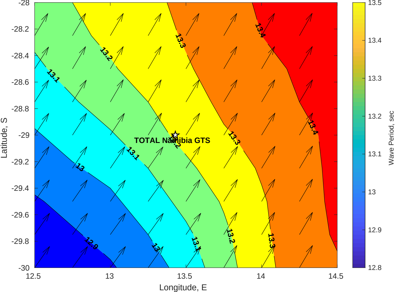
Wave Period (sec) for TOTAL Namibia GTS at 23-May-2025 09:00:00
