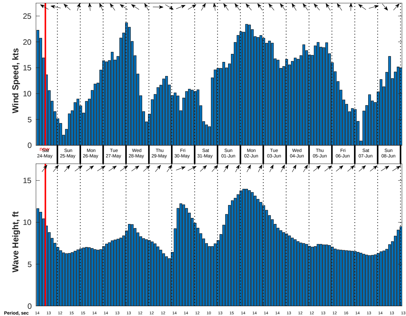
Wind & Wave Forecast for TOTAL Namibia GTS from 23-May-2025 02:00:00 to 08-Jun-2025 02:00:00
