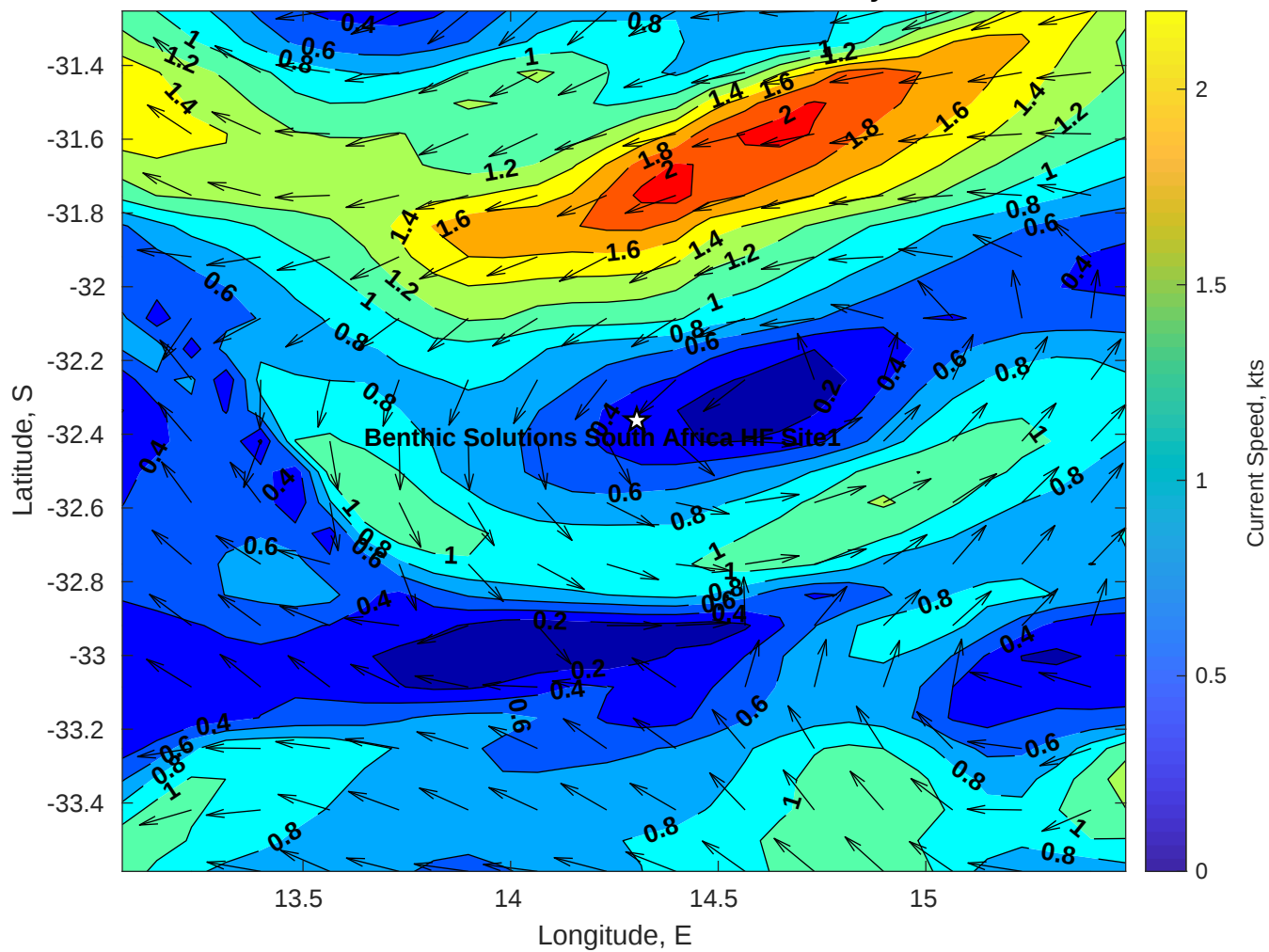
Surface Currents for Benthic Solutions South Africa HF Site1 at 23-May-2025 00:00:00
