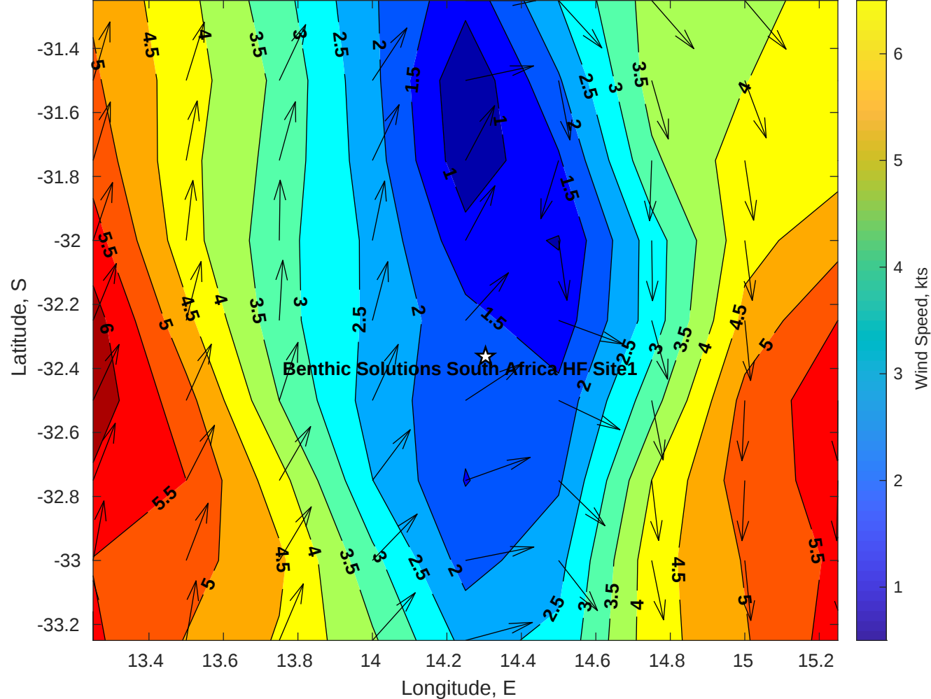
Winds (kts) for Benthic Solutions South Africa HF Site1 at 24-May-2025 09:00:00
