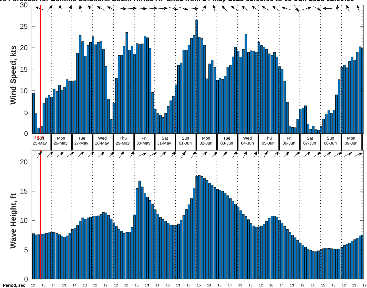
Wind & Wave Forecast for Benthic Solutions South Africa HF Site1 from 24-May-2025 02:00:00 to 09-Jun-2025 02:00:00
