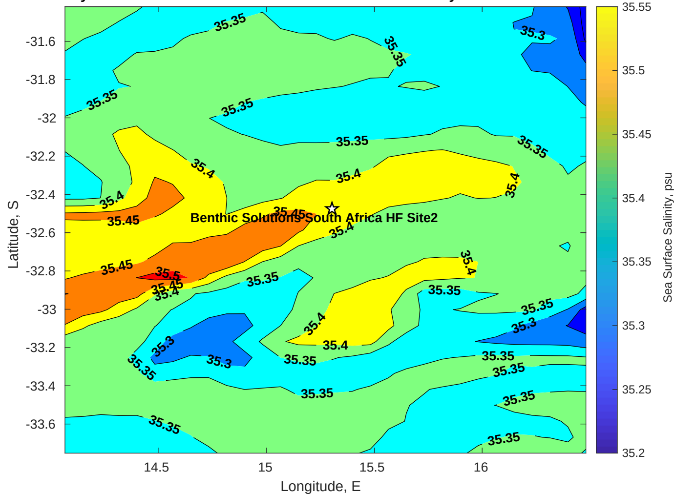
Surface Salinity for Benthic Solutions South Africa HF Site2 at 23-May-2025 00:00:00
