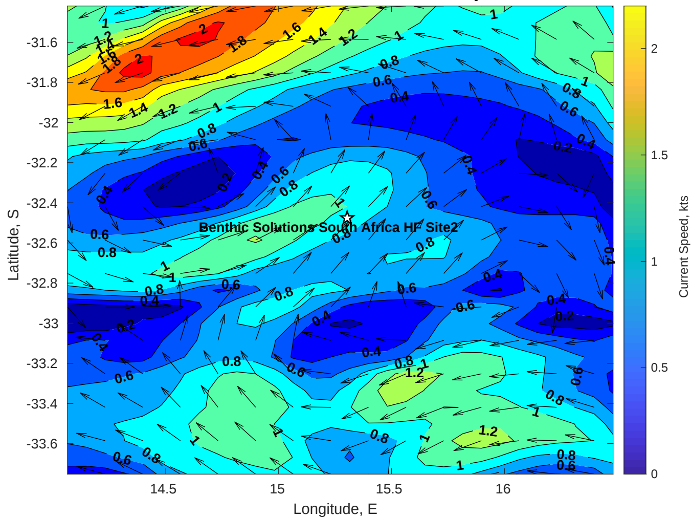
Surface Currents for Benthic Solutions South Africa HF Site2 at 23-May-2025 00:00:00
