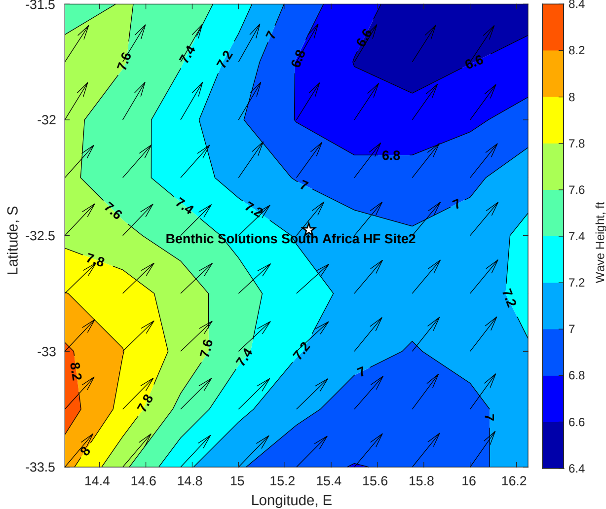
Wave Height (ft) for Benthic Solutions South Africa HF Site2 at 24-May-2025 09:00:00
