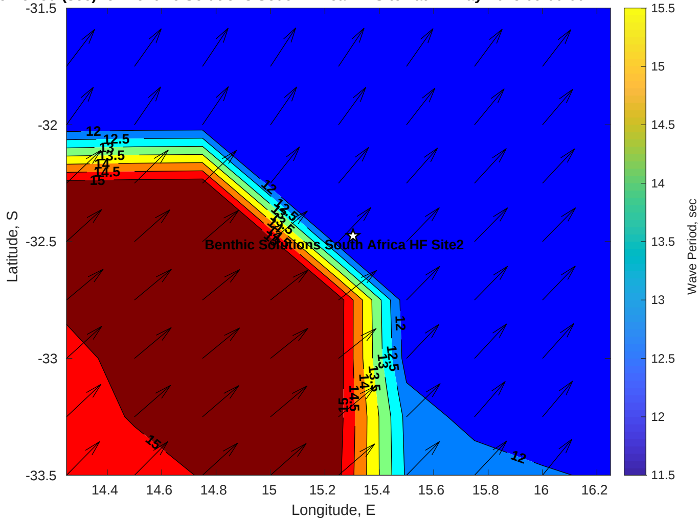
Wave Period (sec) for Benthic Solutions South Africa HF Site2 at 24-May-2025 09:00:00
