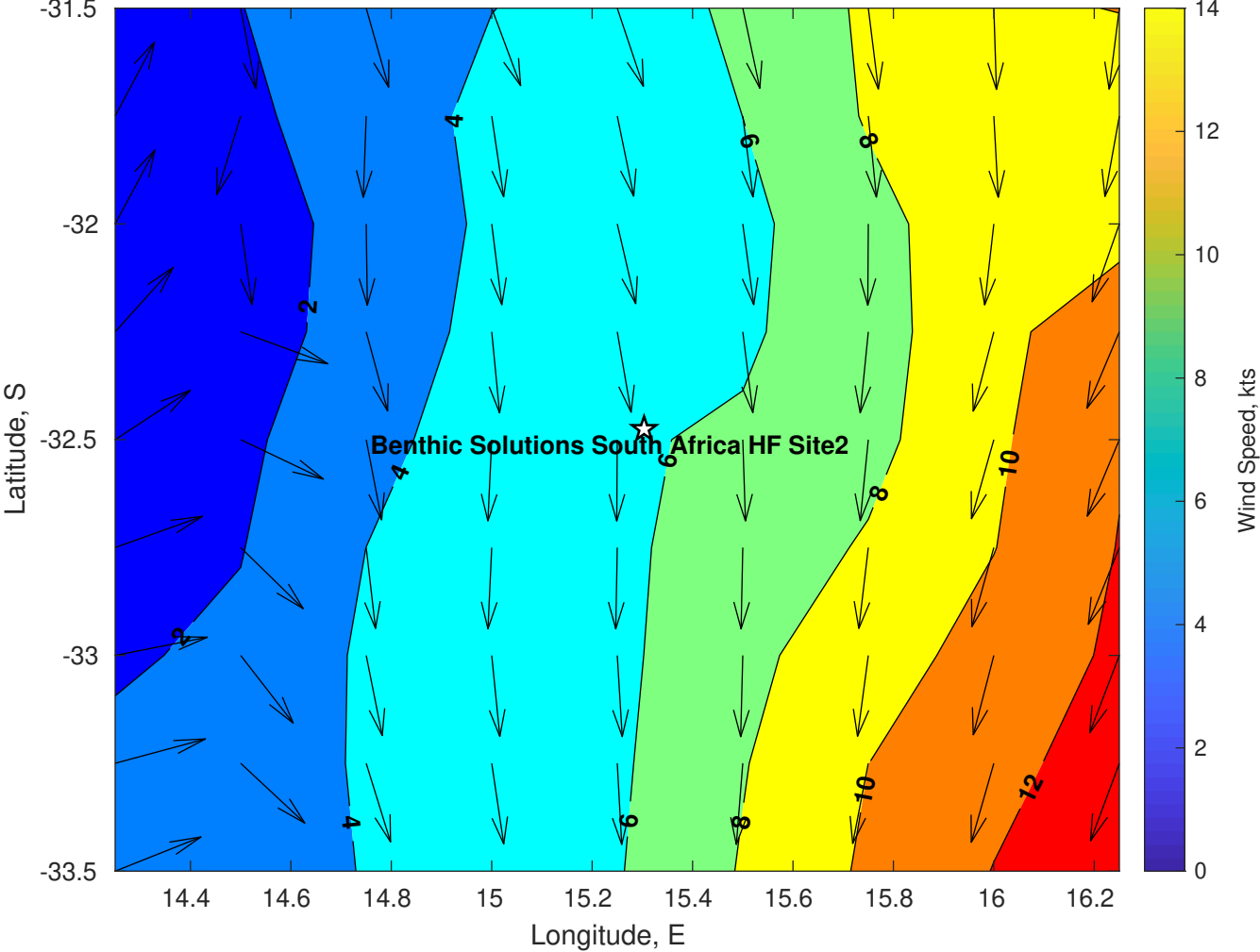
Winds (kts) for Benthic Solutions South Africa HF Site2 at 24-May-2025 09:00:00
