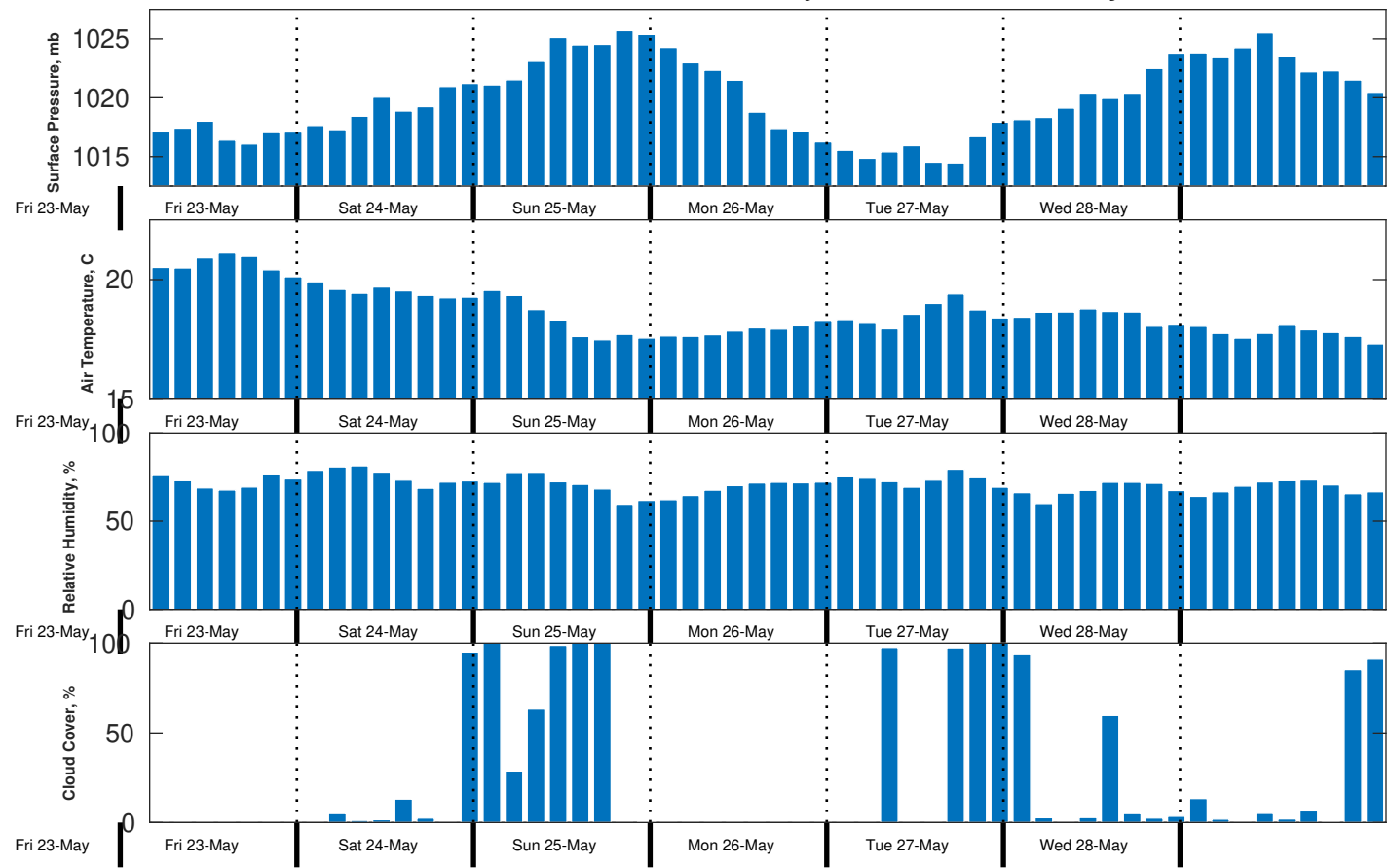
Met Forecast for Benthic Solutions South Africa HF Site2 from 24-May-2025 00:00:00 to 31-May-2025 00:00:00
