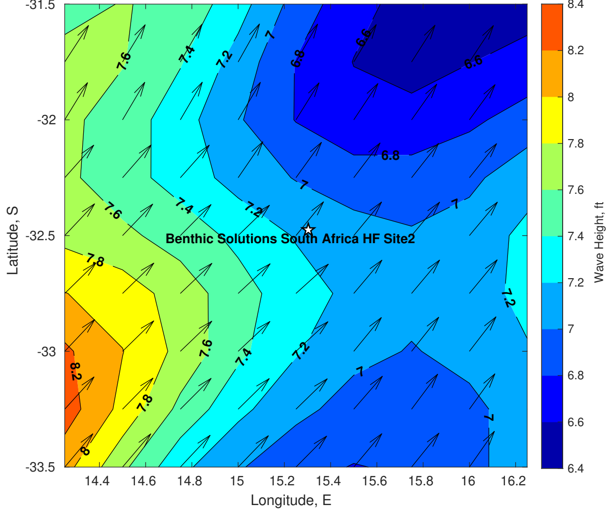
Wave Height (ft) for Benthic Solutions South Africa HF Site2 at 24-May-2025 09:00:00
