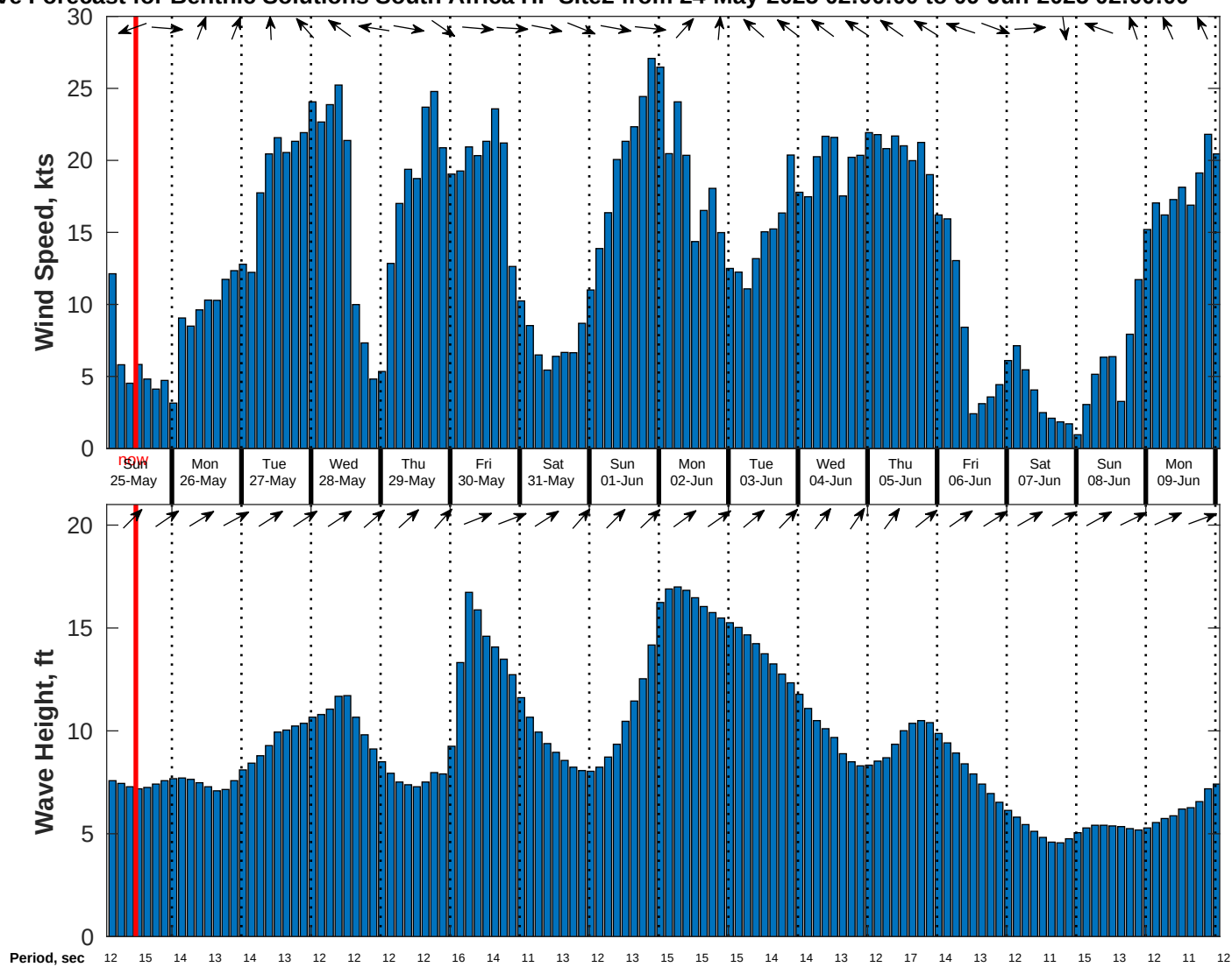
Wind & Wave Forecast for Benthic Solutions South Africa HF Site2 from 24-May-2025 02:00:00 to 09-Jun-2025 02:00:00
