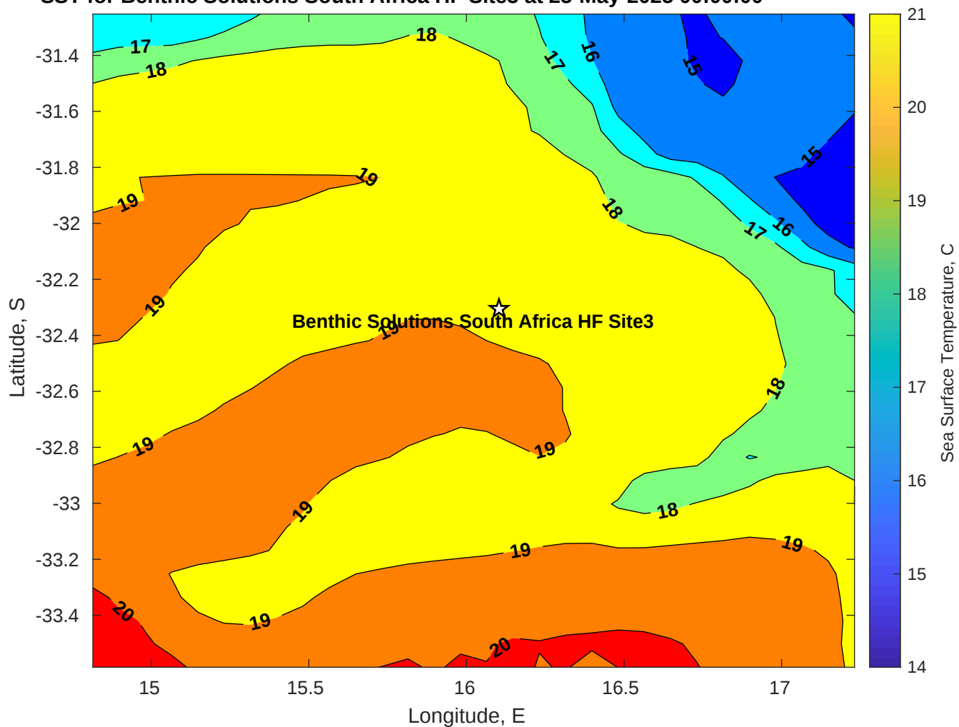
SST for Benthic Solutions South Africa HF Site3 at 23-May-2025 00:00:00
