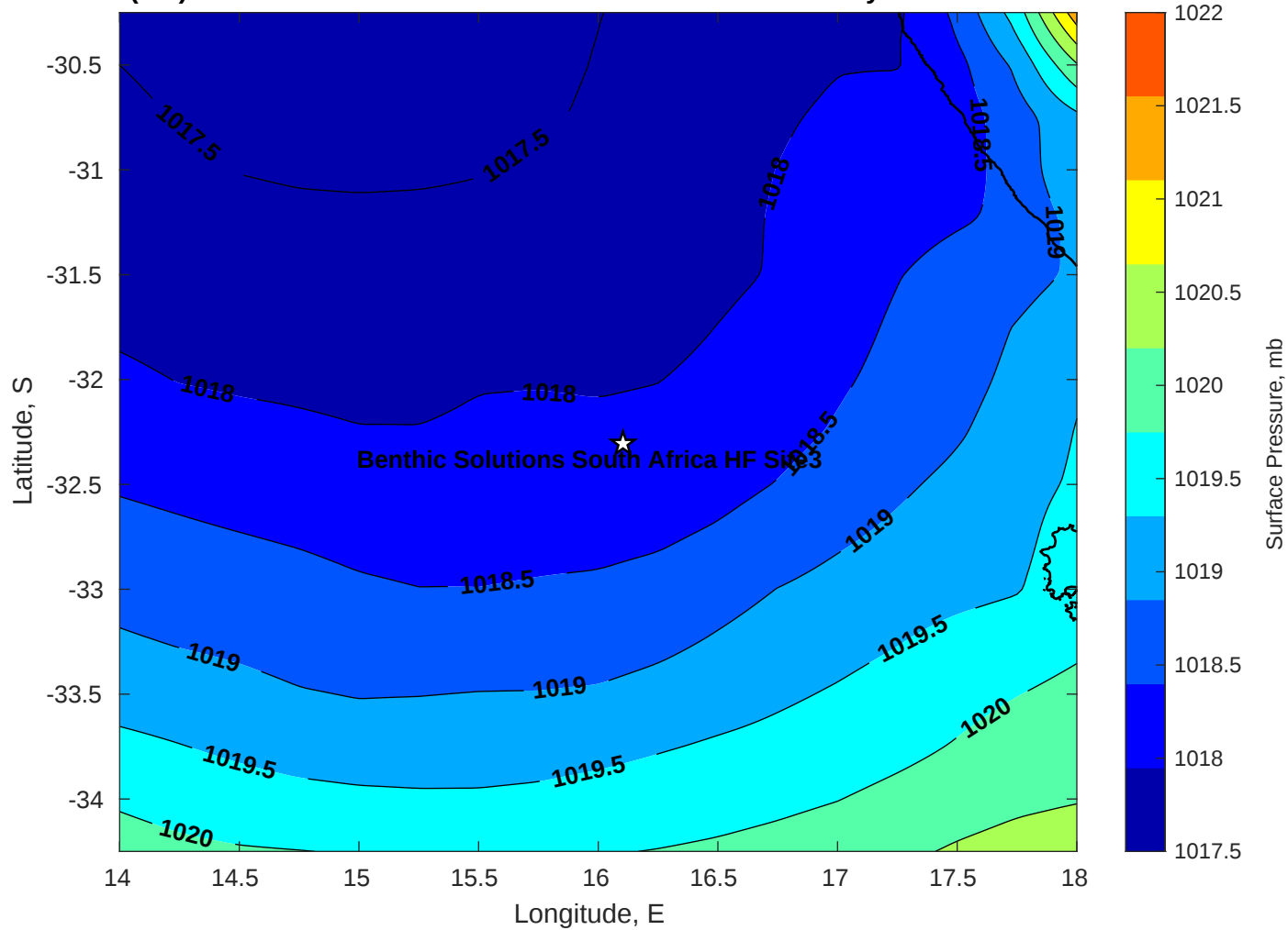
Surface Pressure (mb) for Benthic Solutions South Africa HF Site3 at 24-May-2025 00:00:00
