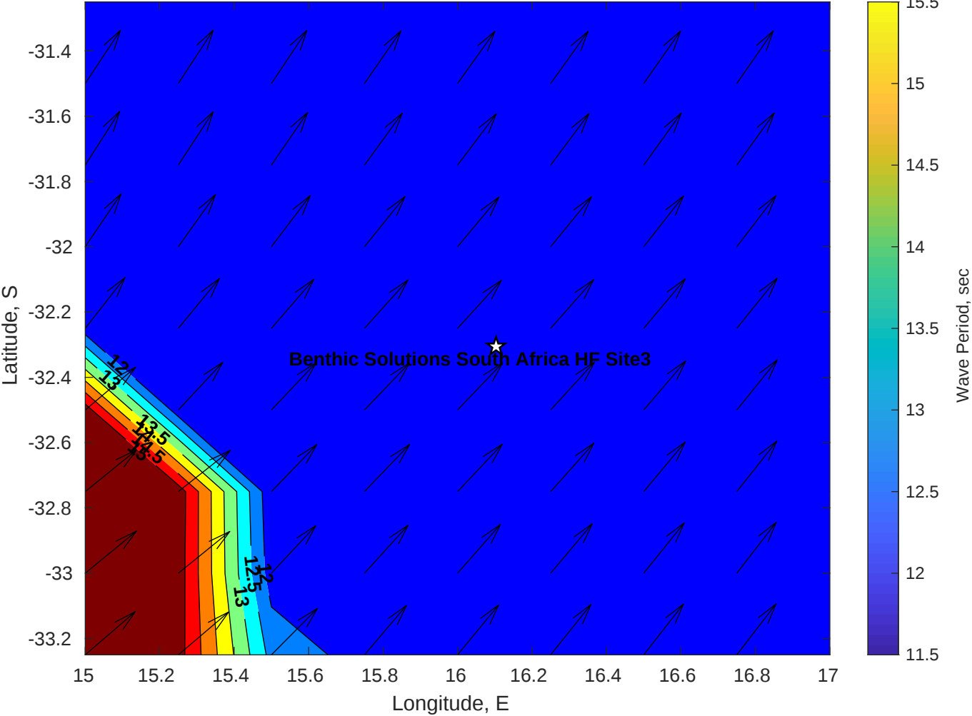
Wave Period (sec) for Benthic Solutions South Africa HF Site3 at 24-May-2025 09:00:00
