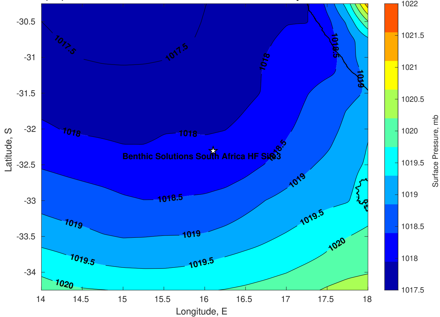
Surface Pressure (mb) for Benthic Solutions South Africa HF Site3 at 24-May-2025 00:00:00
