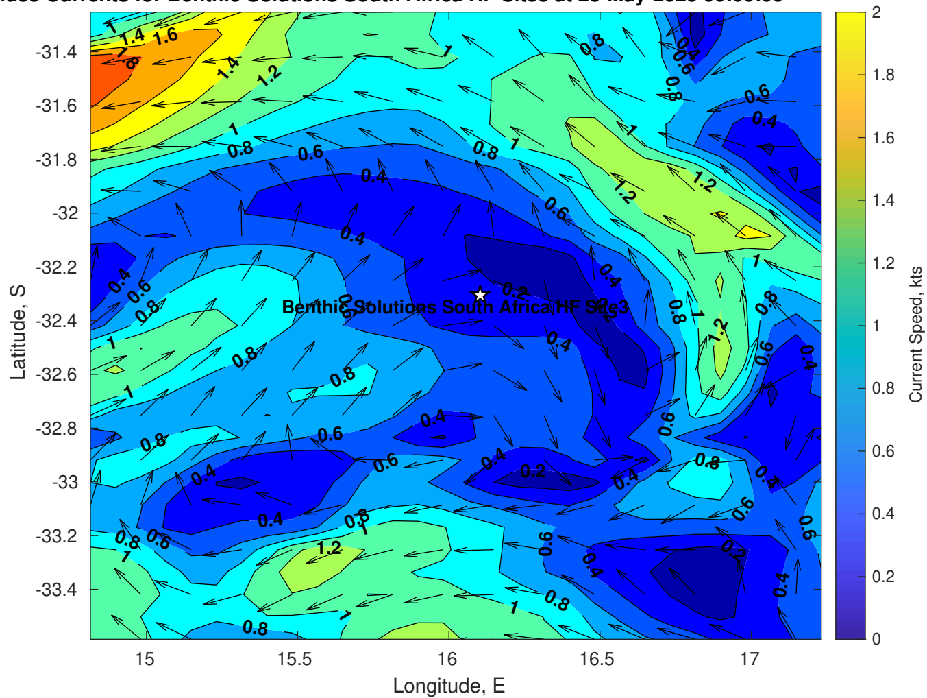
Surface Currents for Benthic Solutions South Africa HF Site3 at 23-May-2025 00:00:00
