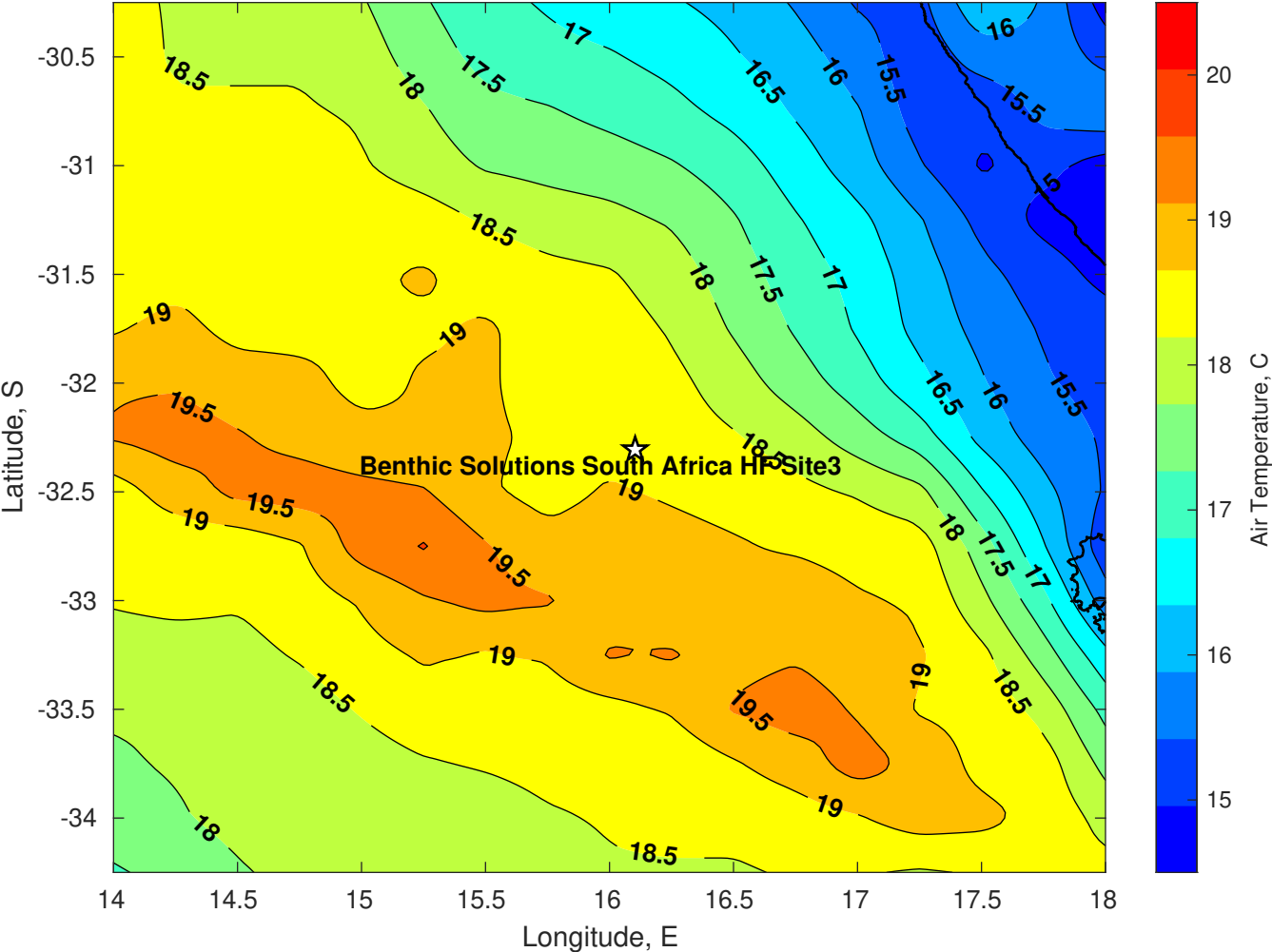
Air Temperature (C) for Benthic Solutions South Africa HF Site3 at 24-May-2025
