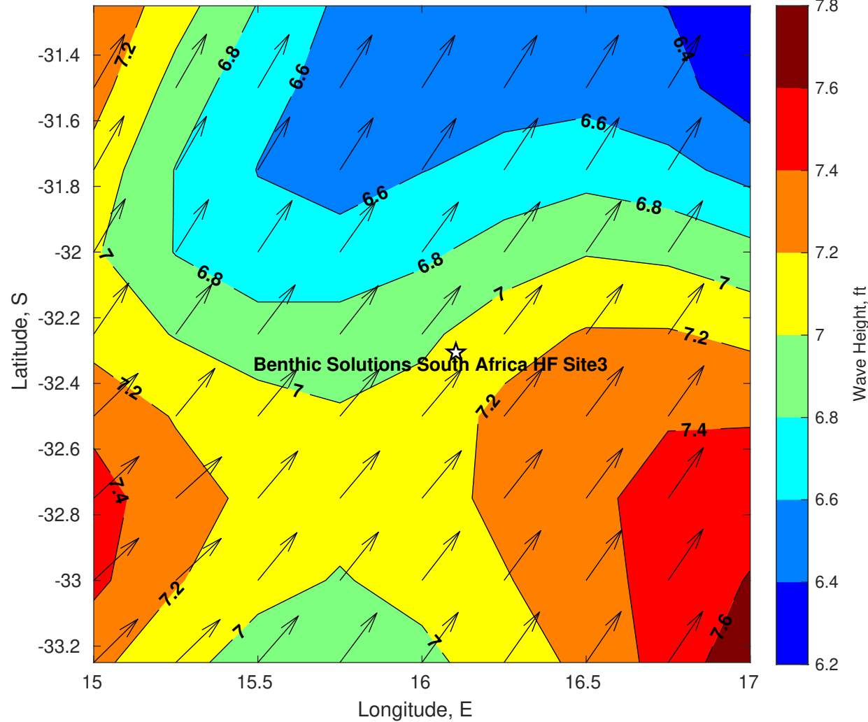
Wave Height (ft) for Benthic Solutions South Africa HF Site3 at 24-May-2025 09:00:00
