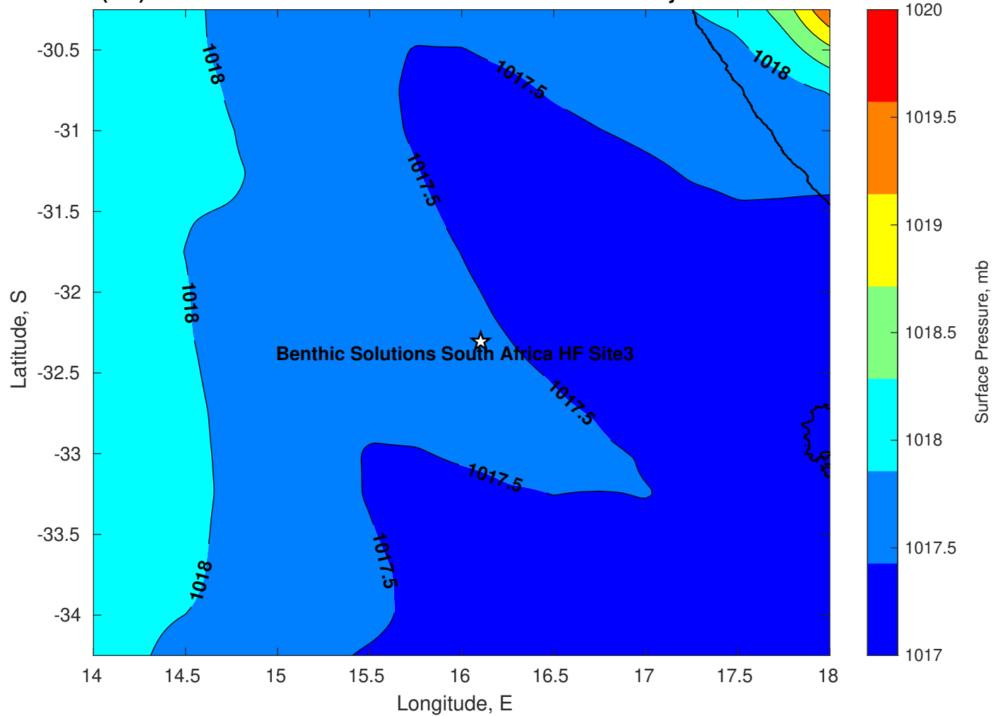
Surface Pressure (mb) for Benthic Solutions South Africa HF Site3 at 25-May-2025 00:00:00
