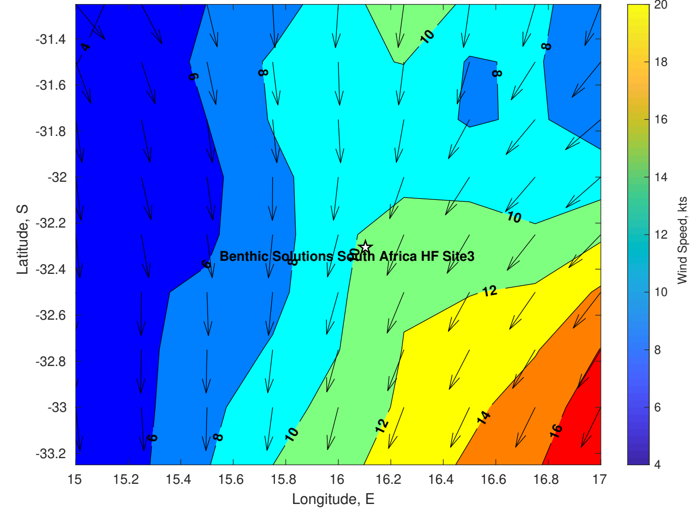
Winds (kts) for Benthic Solutions South Africa HF Site3 at 24-May-2025 09:00:00
