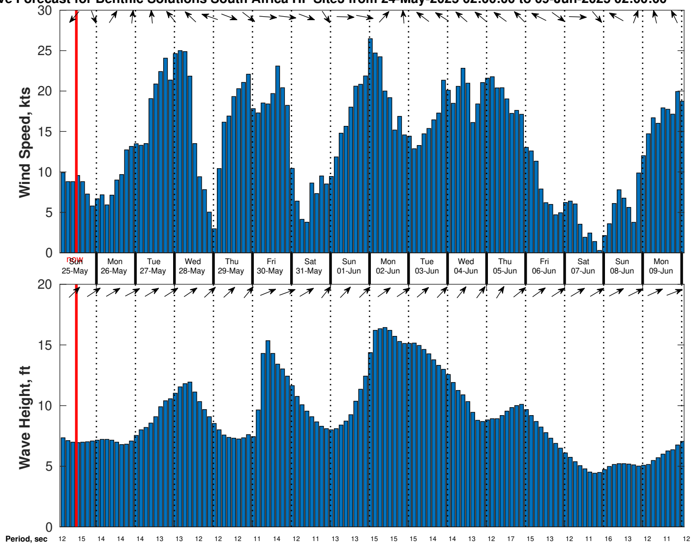
Wind & Wave Forecast for Benthic Solutions South Africa HF Site3 from 24-May-2025 02:00:00 to 09-Jun-2025 02:00:00
