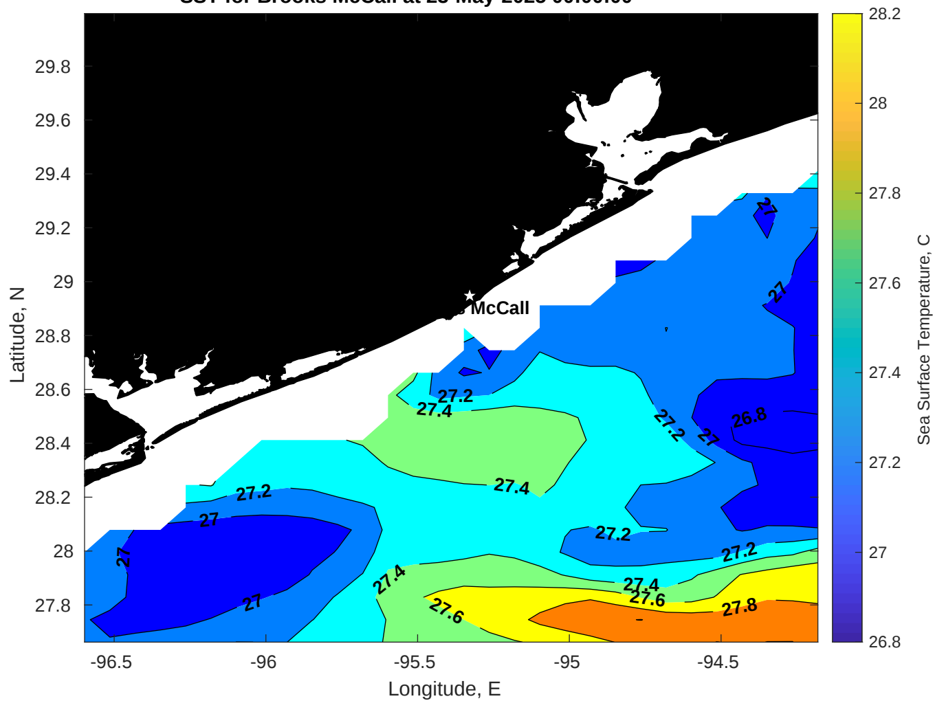
SST for Brooks McCall at 23-May-2025 00:00:00
