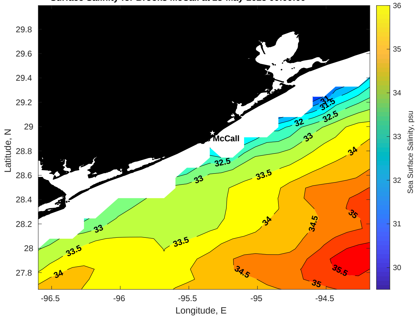
Surface Salinity for Brooks McCall at 23-May-2025 00:00:00
