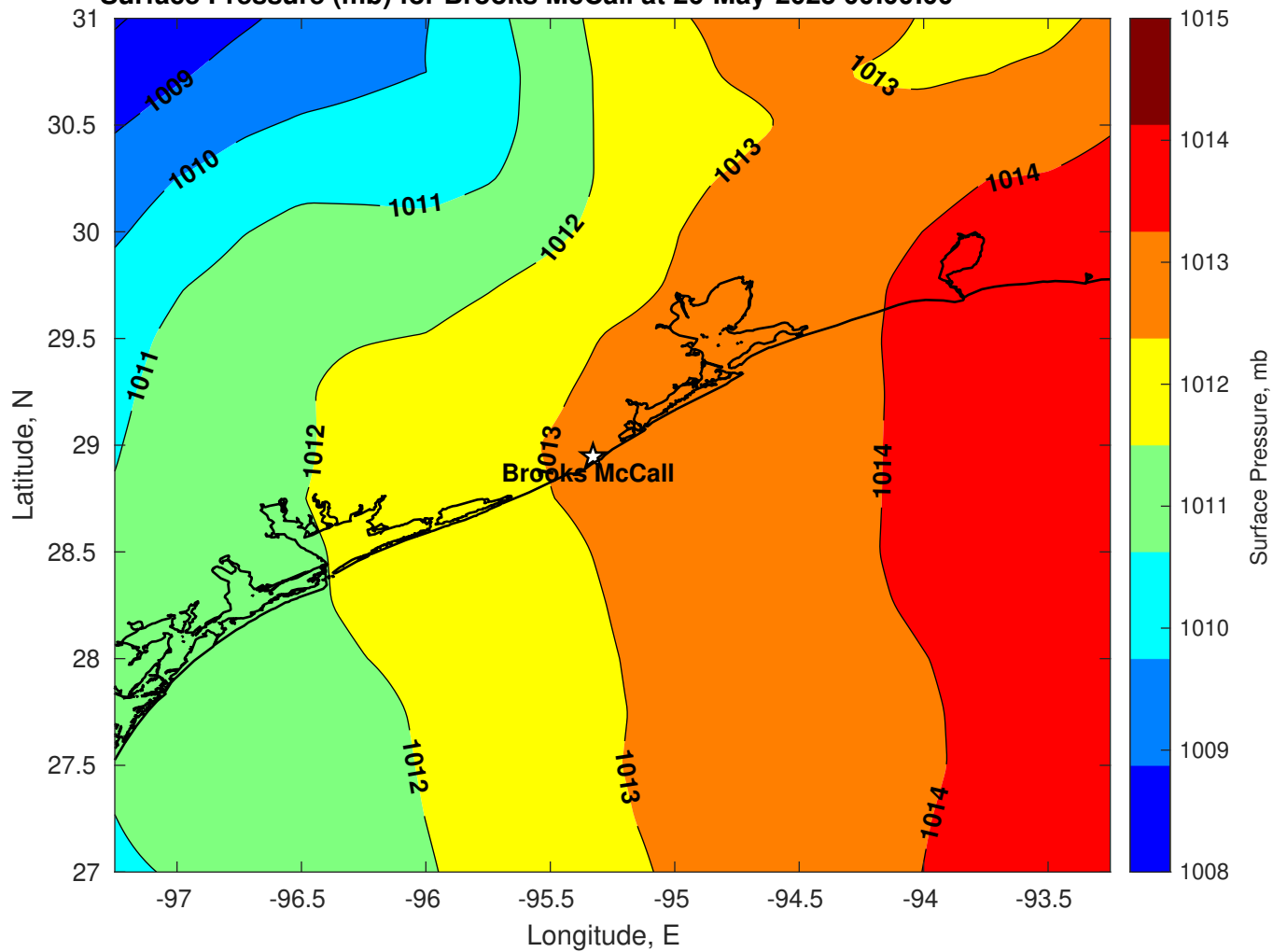
Surface Pressure (mb) for Brooks McCall at 26-May-2025 00:00:00
