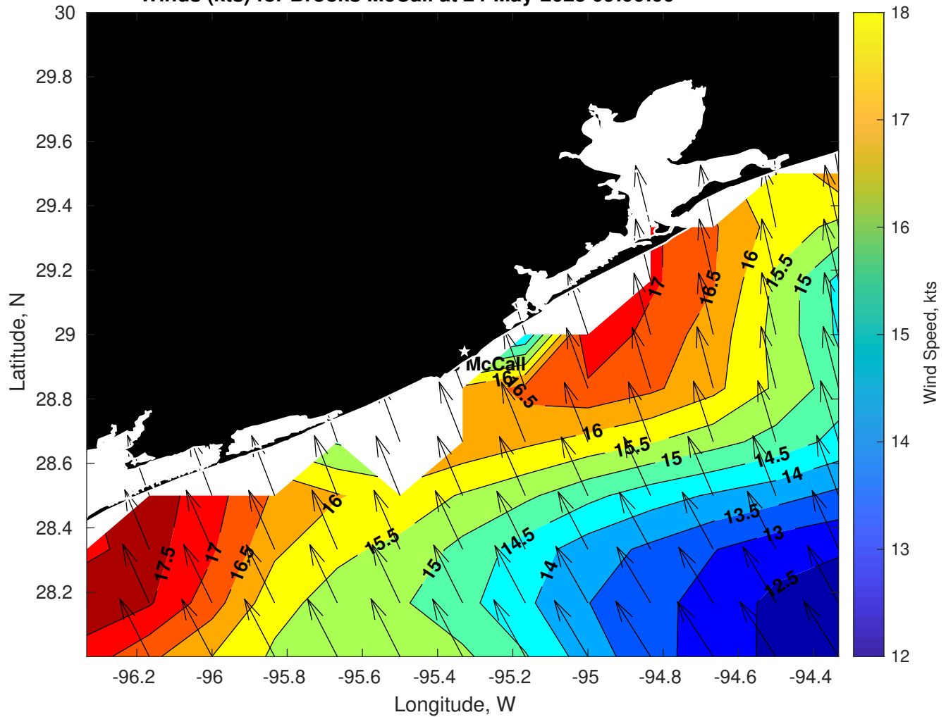
Winds (kts) for Brooks McCall at 24-May-2025 09:00:00
