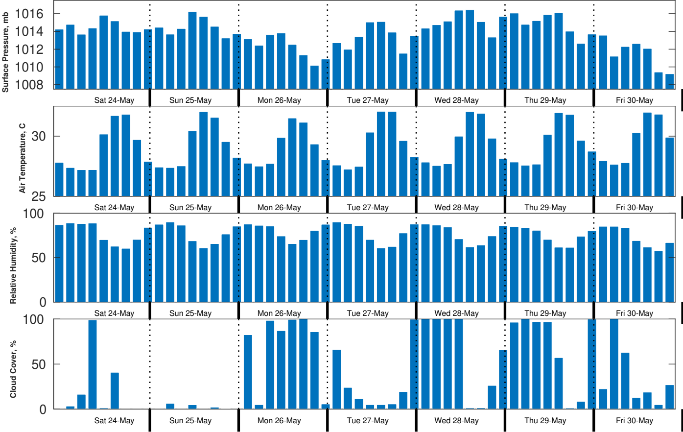
Met Forecast for Brooks McCall from 24-May-2025 00:00:00 to 31-May-2025 00:00:00
