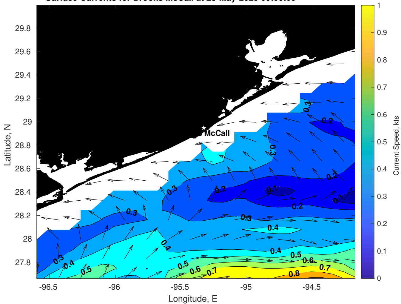
Surface Currents for Brooks McCall at 23-May-2025 00:00:00
