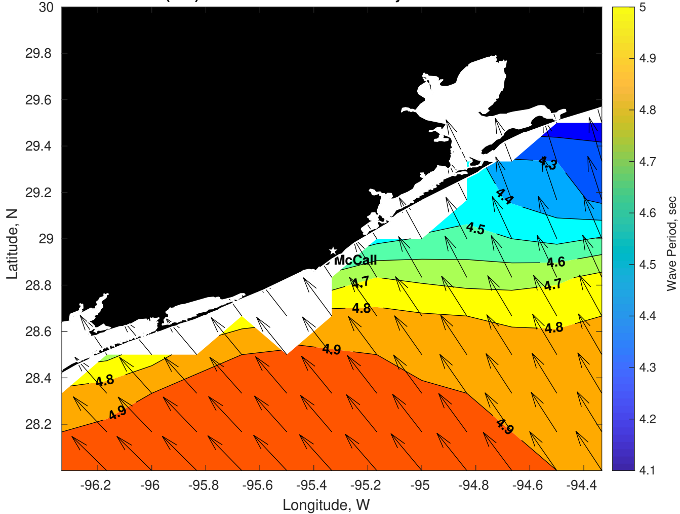
Wave Period (sec) for Brooks McCall at 24-May-2025 09:00:00
